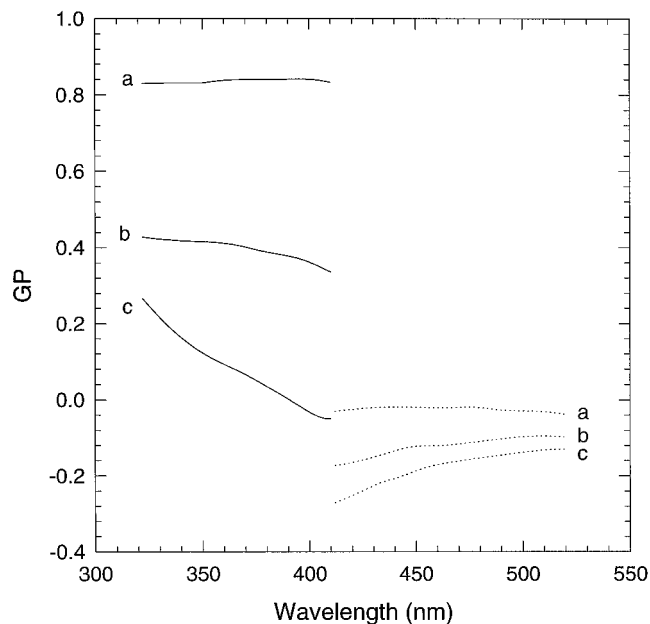
FIGURE 7 GP ex (continuous line) and GP em (dotted line) of LAURDAN in pure GalCer vesicles below ( a ), at ( b ), and above ( c ) the main phase transition temperature. Similar spectra profiles were found in pure Gg 3 Cer, Sulf, Phre, and Sphin vesicles.
