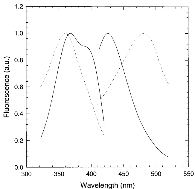
FIGURE 6 Normalized excitation and emission spectra of LAURDAN in pure GalCer vesicles below ( continuous line ) and above ( dotted line ) the main phase transition temperature. The same excitation spectra features were found in pure Gg 3 Cer, Sulf, Phre, and Sphin vesicles.
