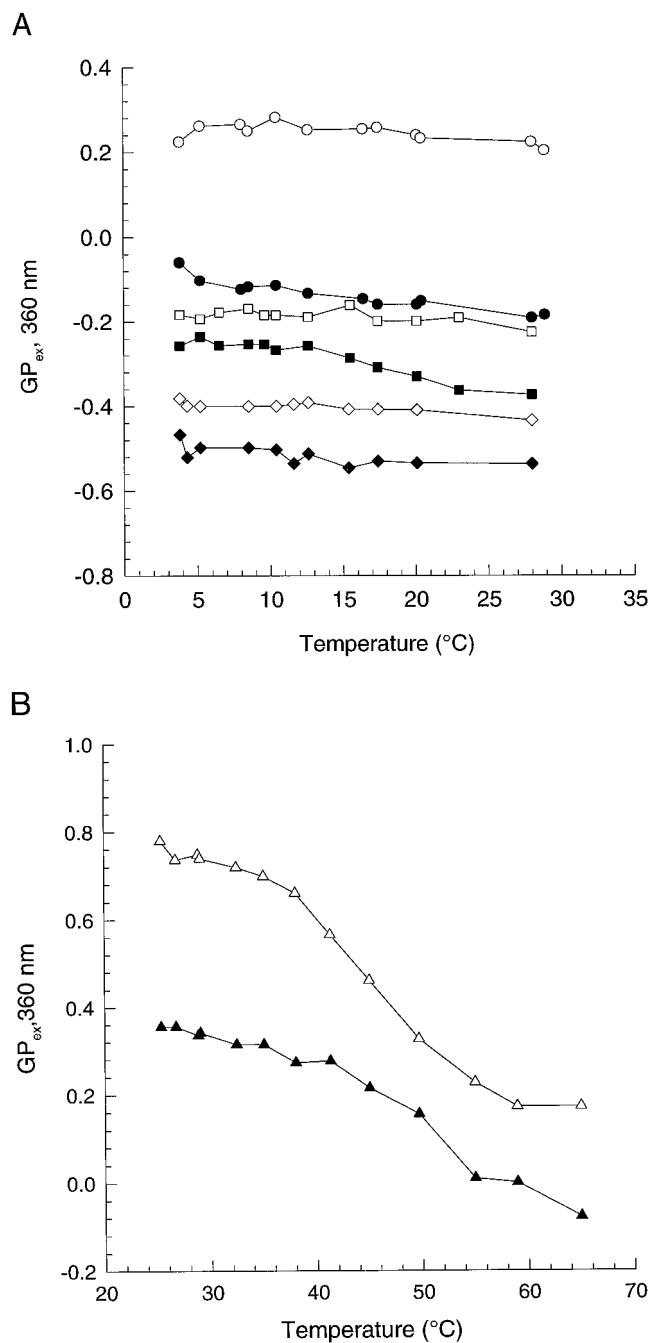
FIGURE 8 GP_{ex} values as a function of temperature for LAURDAN in GSLs aggregates with (empty symbols) and without (filled symbols) cholesterol. (A) G_{T1b} ( \diamond ), G_{D1a} ( \square ), and G_{M1} ( \circ ) micelles, and (B) Gg_4Cer ( \triangle ) vesicles. The GP_{ex} values were calculated using an excitation wavelength of 360 nm. In the mixtures the cholesterol percentage was 20%.
