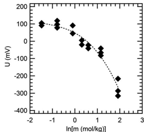
Figure 3. Measured open circuit potential, U , from concentration cells of the form Li | PEO/LiTFSI ( r_{\text{ref}} ) | PEO/LiTFSI ( r ) | Li at 90°C. Here, r_{\text{ref}} is the reference held at r = 0.06 , and r is varied. Each point represents data from one concentration cell. The dashed line shows the polynomial fit given by Eq. 13.
