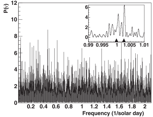
FIG. 3. Periodogram for opposite-sign dilepton events. The solar-day and sidereal-day frequencies, indicated by the left and right triangles (inset), are well resolved in our data.
