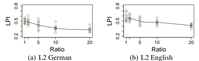
Figure 3: Final level of L2 proficiency ( LPI ) in each simulation for different R values, with LOESS curves fitted
