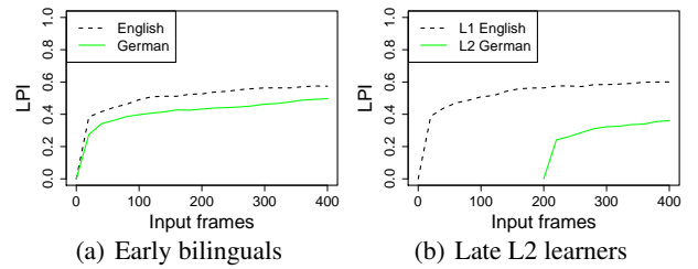
Figure 1: LPI change over time in two specific settings ence between English and German data sets – as mentioned before, the total number of values for arguments' role properties is larger in the German data set, which makes the task of predicting this feature more difficult in German than in English. However, a combination of larger R and AO can reverse this effect. In the late L2 learning scenario (Figure 1(b)) the lower level of L2 proficiency could be caused both by different R and AO values. The following experiments investigate the impact of each of the two variables in isolation.
