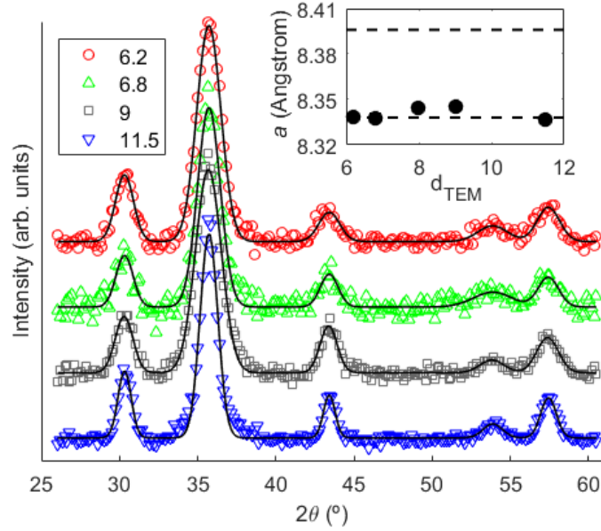
Figure S4. X-ray diffraction patterns from iron oxide cores of the VCD sample series; the values in the legend are the corresponding TEM diameters in nanometers. The data have been background corrected. The solid line curves are fits obtained using profile-matching based on the allowed Bragg reflections for maghemite over the measured 2\theta range; i.e., from left to right, the (2 2 0), (3 1 1), (4 0 0), (4 2 2) and (5 1 1). The resulting (fitted) lattice parameter values are presented in the inset, where the errors bars are smaller than the plotted points. The lattice parameter at d_{\text{TEM}} = 8 nm is taken from a similar analysis. 14 The lower and upper horizontal dashed lines in the inset indicate the bulk lattice parameter values of maghemite and magnetite, respectively.
