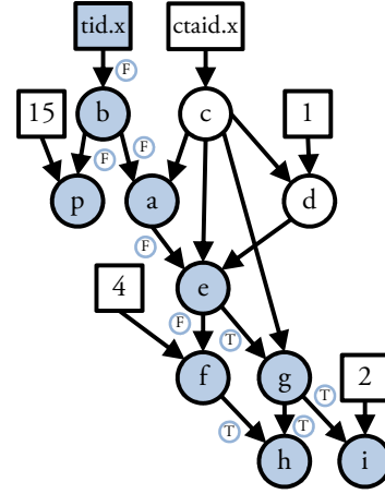
(b) Resulting graph.
