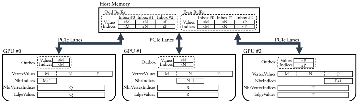
Figure 2.8: Organization of data structures in multi-GPU processing.
