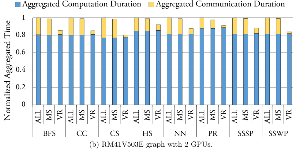
Figure 2.11: Processing-time break down into computation time and communication time for the Vertex Refinement (VR) compared to ALL and MS. Computation time is the total duration of kernel execution, and communication time is the total duration of inbox/outbox management plus inter-device memory copies. For each benchmark, the times are normalized with respect to the longest time. Note that this times cannot be used to infer the overall speedup due to asynchronicity of devices.
