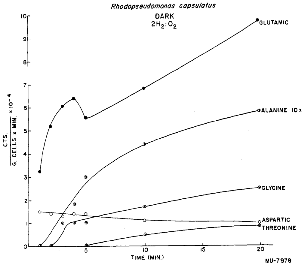
Fig. 12 C 14 distribution in amino acids after C 14 O 2 fixation by Rhodopseudomonas capsulatus in the dark. 44 mg/ml cells. 41 ml suspension. 2H 2 : O 2 in the gaseous space.
