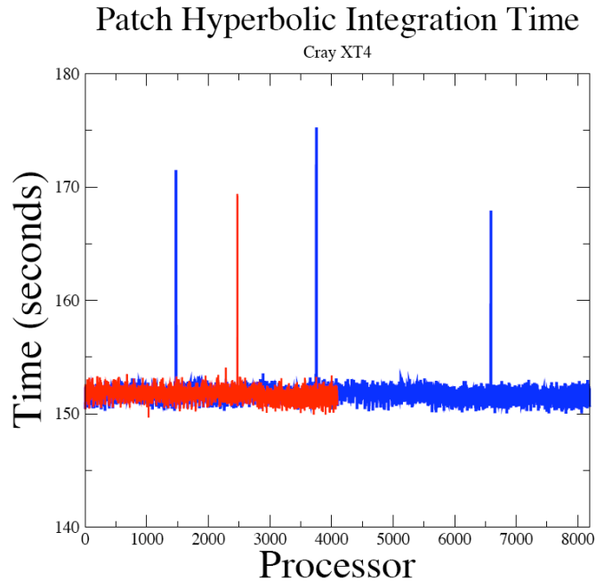
Figure 10. Variation in loads for large numbers of processors. Red (4096 processor calculation) and blue (8192 processor calculation) show the time spent in the patch update as a function of processor number on a union of fixed-size patches for an unsplit PPM algorithm. The spikes correspond to specific hardware nodes, and were found to be caused by single-bit errors in the memory on those nodes [3].
