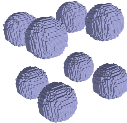
Figure 5. Spherical shell grids replicated by a factor of two in each coordinate direction.
