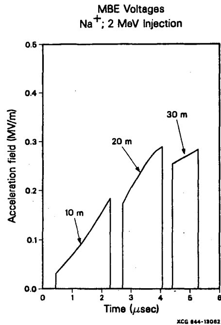
Fig. 4. Accelerating voltage waveforms at 10 m, 20 m, and 30 m, along the length of the MBE accelerator.
