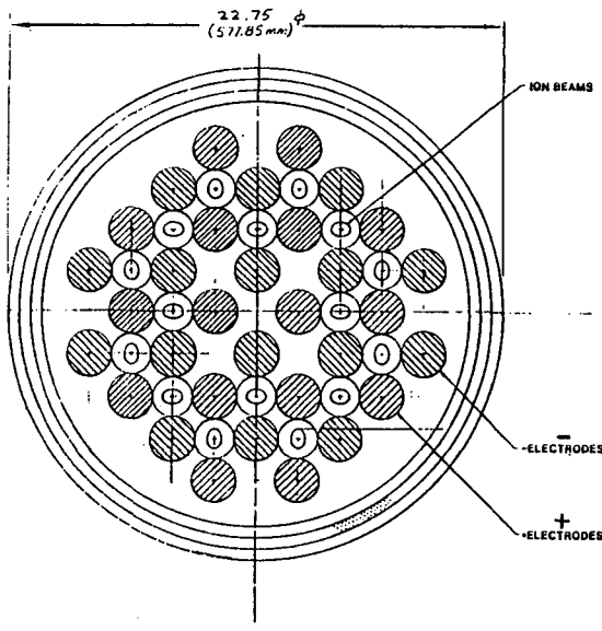
Fig. 6. Axial section of the MBE quadrupole focussing array.
