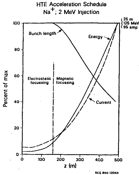
Fig. 1 Acceleration and compression schedule for the HTE accelerator.
