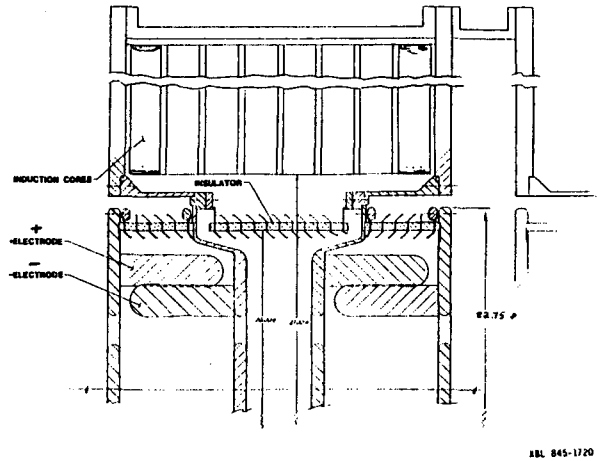
Fig. 7. Cross section of an MBE induction unit.
