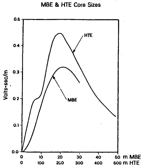
Fig. 5. Volt-sec/m needed for the HTE and MBE accelerators. The abscissa is 100 m/div for HTE and 10 m/div for MBE. The ordinate is 0.1 volt-sec/m for both.
