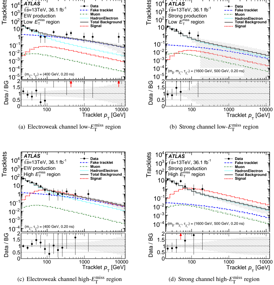
Figure 7: Pixel-tracklet p_T spectrum in various regions: (a) electroweak channel in the low- E_T^{\text{miss}} region, (b) strong channel in the low- E_T^{\text{miss}} region, (c) electroweak channel in the high- E_T^{\text{miss}} region, and (d) strong channel in the high- E_T^{\text{miss}} region. Observed data are shown with markers and the background components for the background-only fit are shown with lines. In the strong channel, total background lines overlap hadron and electron background lines. An example of the expected signal spectrum at \tau_{\tilde{\chi}_1^\pm} = 0.2 ns and m_{\tilde{\chi}_1^\pm} = 400 GeV for the electroweak channel and m_{\tilde{g}} = 1600 GeV, m_{\tilde{\chi}_1^\pm} = 500 GeV for the strong channel is overlaid for comparison. The bottom panels show the ratio of the data to the background predictions. The error band shows the uncertainty in the background prediction including both the statistical and systematic uncertainties. Red arrows in the Data/BG ratio indicate bins where the corresponding entry falls outside the plotted range.
