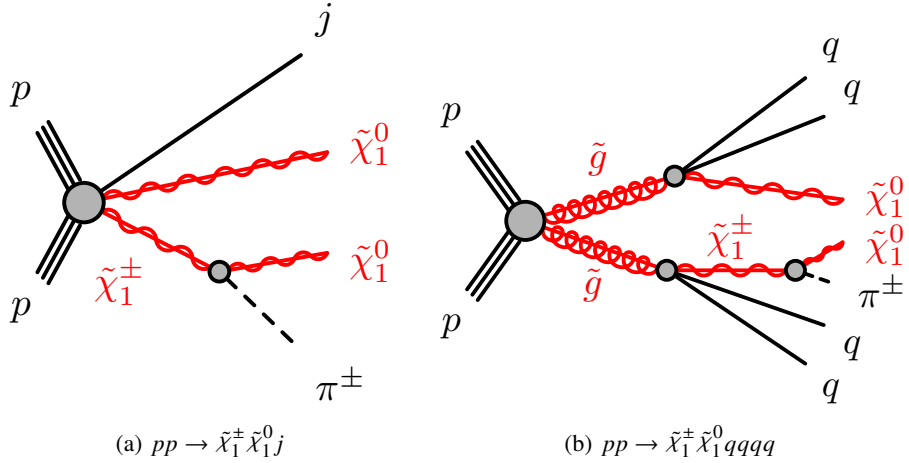
Figure 2: Example diagrams of the benchmark signal processes used in this analysis. In the case of direct chargino/neutralino production (a), the signal signature consists of a long-lived chargino, missing transverse momentum and initial-state radiation. In the case of the strong channel (b), each gluino decays into two quarks and a chargino or neutralino. A long-lived chargino, missing transverse momentum and multiple quarks, which are observed as jets, are the signatures of this signal.
