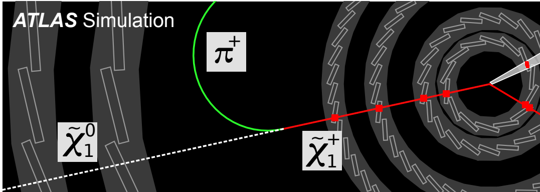
Figure 1: Illustration of a pp \rightarrow \tilde{\chi}_1^+ \tilde{\chi}_1^- + \text{jet} event, with long-lived charginos. Particles produced in pile-up pp interactions are not shown. The \tilde{\chi}_1^+ decays into a low-momentum pion and a \tilde{\chi}_1^0 after leaving hits in the four pixel layers (indicated by red markers).
