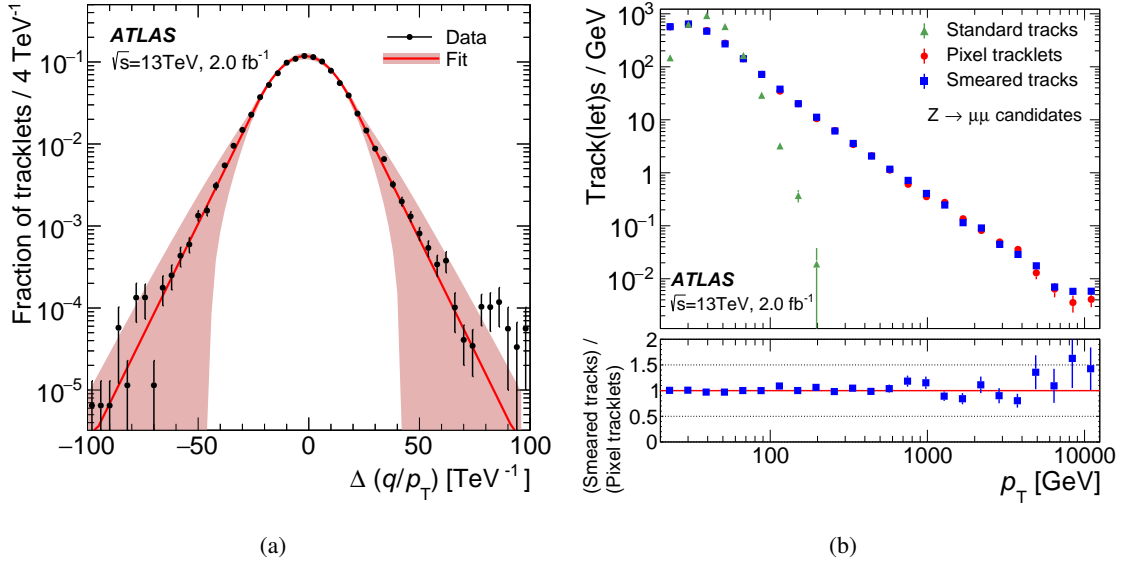
Figure 5: (a) Distribution of the difference between q/p_T of a pixel tracklet and a track in Z \rightarrow \mu\mu events in data. The solid curve shows the smearing function (eq. (1)) used to construct the background p_T template, which is described in section 6.1. The parameter values of the curve are \alpha = 1.67 , \beta = -1.72 \text{ TeV}^{-1} and \sigma = 13.2 \text{ TeV}^{-1} . The red band indicates a 1\sigma variation of the systematic uncertainty (see section 7). The data are normalised to unit area. (b) Validation of the smearing procedure in Z \rightarrow \mu\mu events in data. The green and red points show the p_T distributions of tracks and pixel tracklets respectively. The blue point shows the p_T spectrum obtained by convolving the track p_T distribution with the smearing function. The lower plot shows the ratio of the smeared spectrum to the distribution of the pixel tracklets.
