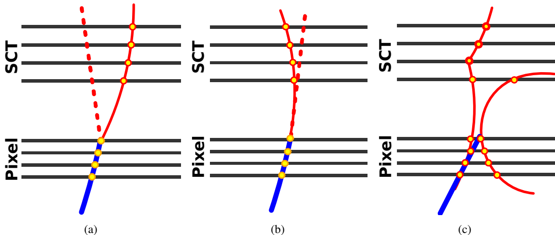
Figure 3: Sketch of the different background components in the search with pixel tracklets. Thin solid and dotted red lines show trajectories of charged and neutral particles respectively. Thick blue lines show reconstructed pixel tracklets. (a) A hadron undergoing a hard scattering can yield track segments in the pixel and SCT detector that are not recognised as belonging to the same track, thus faking a pixel tracklet. (b) A lepton emitting hard photon radiation could be identified as a pixel tracklet through a similar mechanism. (c) A pixel tracklet can arise from a random combination of hits created by different particles in close proximity.
