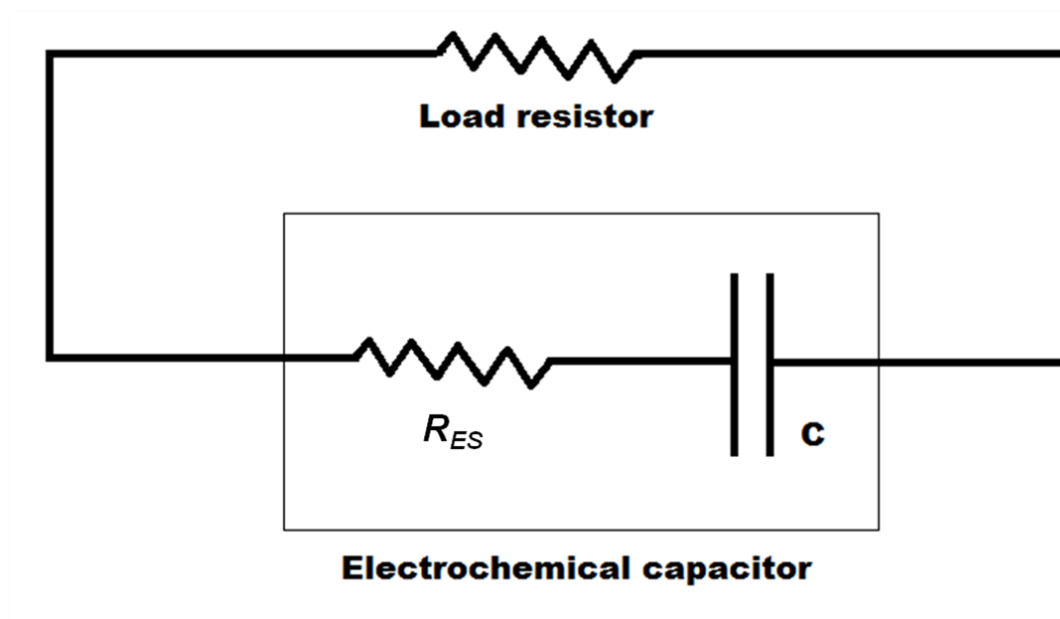
Figure 8. The series RC circuit for supercapacitors.
