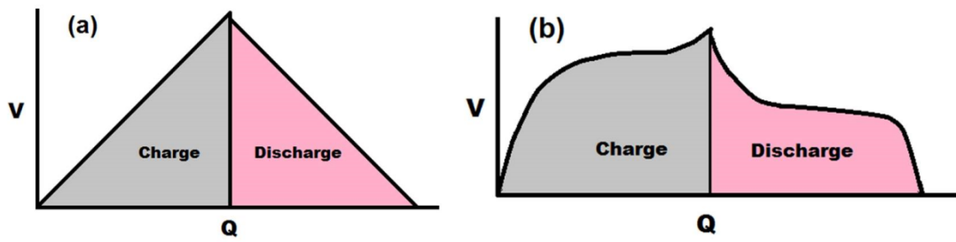
Figure 15. Representative working diagram from CCCD test for EDLCs (a), and PCs (b).
