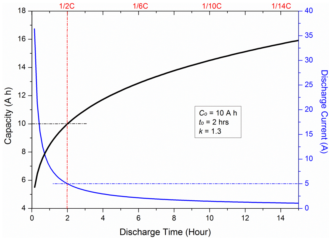
Figure 16. An illustration of Peukert's curve for batteries with the use of \frac{1}{2}C marked by dashed lines.
