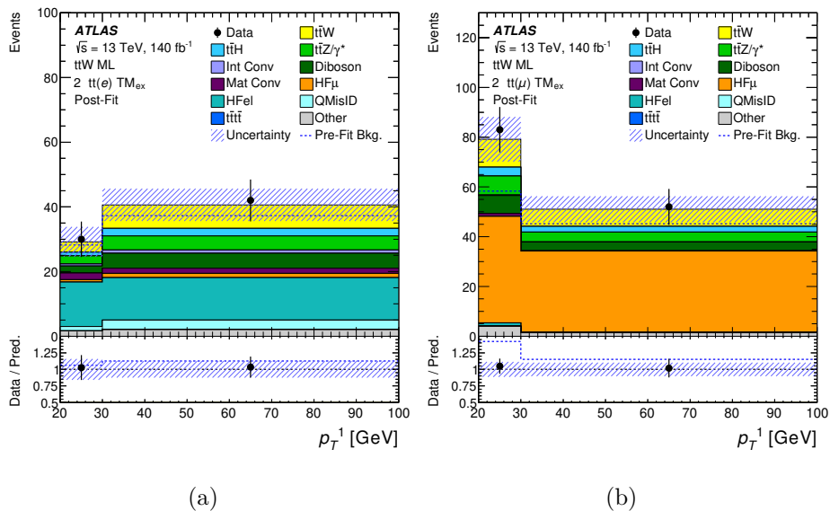
Figure 3. Comparison between data and the signal-plus-background prediction for the distribution of the transverse momentum of the sub-leading lepton ( p_T^{\ell 1} ) in (a) the 2l tt(e)_{TM_{ex}} CR and (b) the 2l tt(\mu)_{TM_{ex}} CR. The signal and background contributions after the likelihood fit to data (“Post-Fit”) under the signal-plus-background hypothesis are shown as filled histograms. The total signal-plus-background prediction before the likelihood fit to data (“Pre-Fit Bkg.”) is shown as a dashed blue histogram in the upper panel. The ratio of the data to the total prediction (“Pred.”) is shown in the lower panel, separately for the post-fit prediction (black points) and pre-fit background (dashed blue line). The combined statistical and systematic uncertainty in the prediction is indicated by the blue hatched band. The last bin in each figure contains the overflow.
