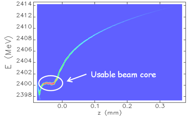
Figure 3: Beam longitudinal phase space at the entrance of the FEL beamlines. (Elegant simulations.)
