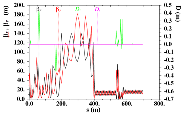
Figure 1: Lattice functions from the exit of the injector through the linac, including switchyard, branchline, and the self-seeded FEL beamline through the last undulator.
