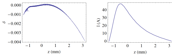
Figure 2: Example of beam longitudinal phase space (left) and current profile at the exit of the injector. The bunch head on the left. (ASTRA simulations).
