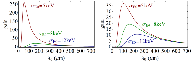
Figure 6: Gain for the microbunching instability from the injector through the last compressor for two-stage (left) and one-stage compression.
