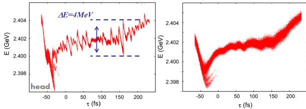
Figure 5: Longitudinal phase-space of the beam core at the exit of the spreader with laser heater off (left) and on. (IMPACT simulations.)
