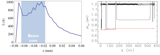
Figure 4: Beam current profile (left) and evolution of the projected transverse rms emittances along the machine.
