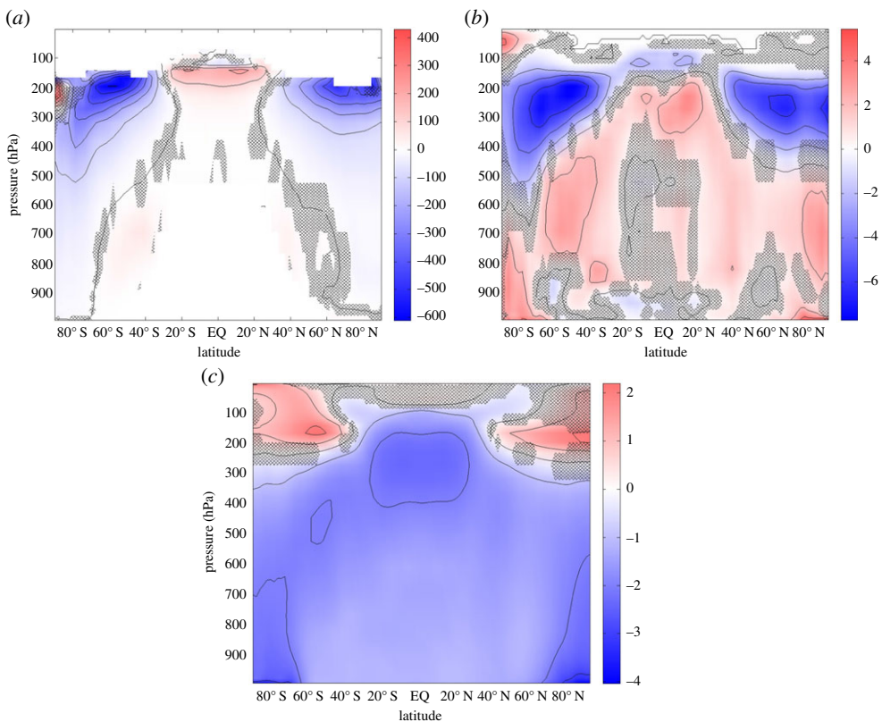
Figure 3. (a) The reduction in in-cloud ice crystal number concentration ( l^{-1} ) in response to seeding (SEEDING — CONTROL), and the corresponding changes in (b) cloud cover (%) and (c) temperature (K). The hatching indicates regions where the difference between SEEDING and CONTROL is not statistically significant (applying a Student's t -test with a significance level of 5%).
