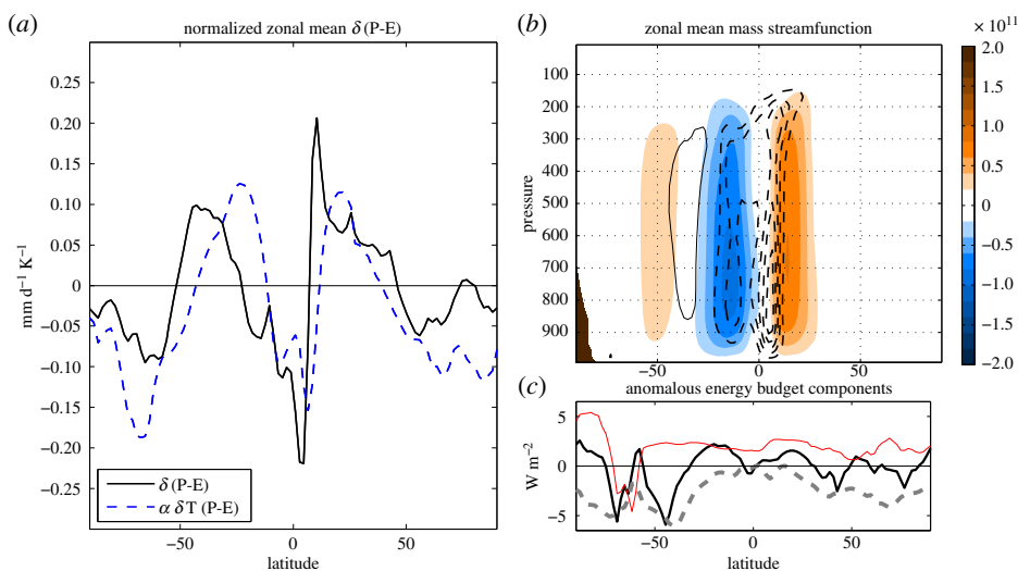
Figure 5. (a) Anomalous (SEEDING — CONTROL) zonal mean simulated rate of precipitation minus rate of evaporation (P-E, solid line), and the anomalous P-E predicted by the thermodynamic scaling, both in millimetres per day. (b) Total zonal mean mass streamfunction in the control run (colour shading, contour interval 10^{10} \text{ kg s}^{-1} ) and anomalous zonal mean mass streamfunction (black contours, negative dashed, interval 2 \times 10^9 \text{ kg s}^{-1} , zero contour not shown). Negative contours signify counterclockwise rotation and the black region near the south pole represents topography. (c) Anomalous clear-sky TOA radiative flux (red line, positive downward), anomalous TOA net cloud radiative forcing (dashed line) and anomalous vertically integrated source of atmospheric MSE (thick black line).
