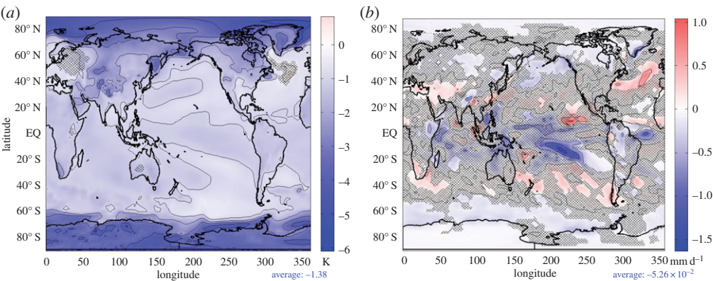
Figure 4. (a) The surface air temperature response to seeding (K) and (b) the corresponding change in total (convective and large-scale) precipitation rate (millimetres per day). The hatching indicates regions where the difference between SEEDING and CONTROL is not statistically significant (based on Student's t -test with a significance level of 5%).
