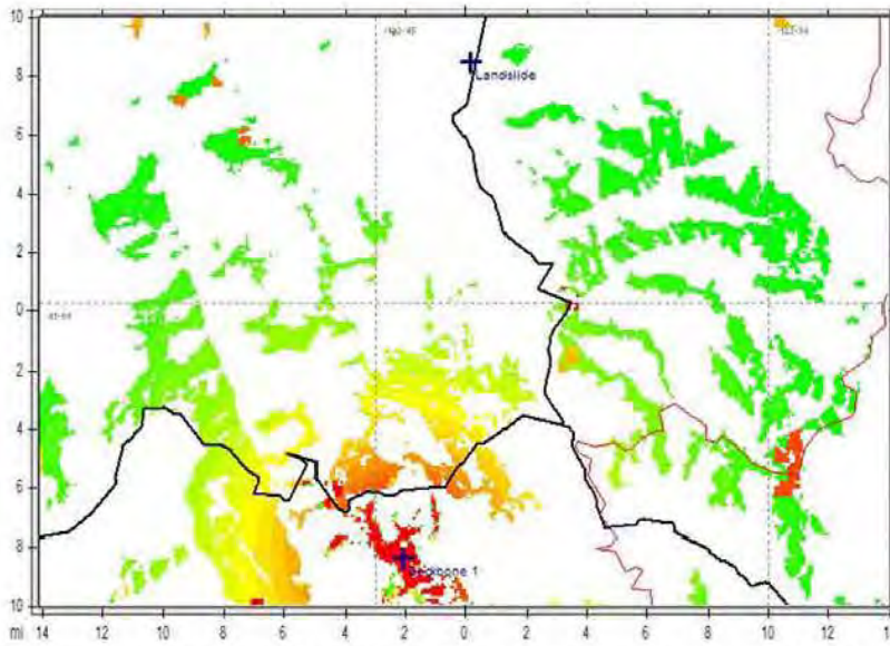
Figure 11: RF Coverage Plot from the nearest State Tower Operating in the 700 MHz Band
