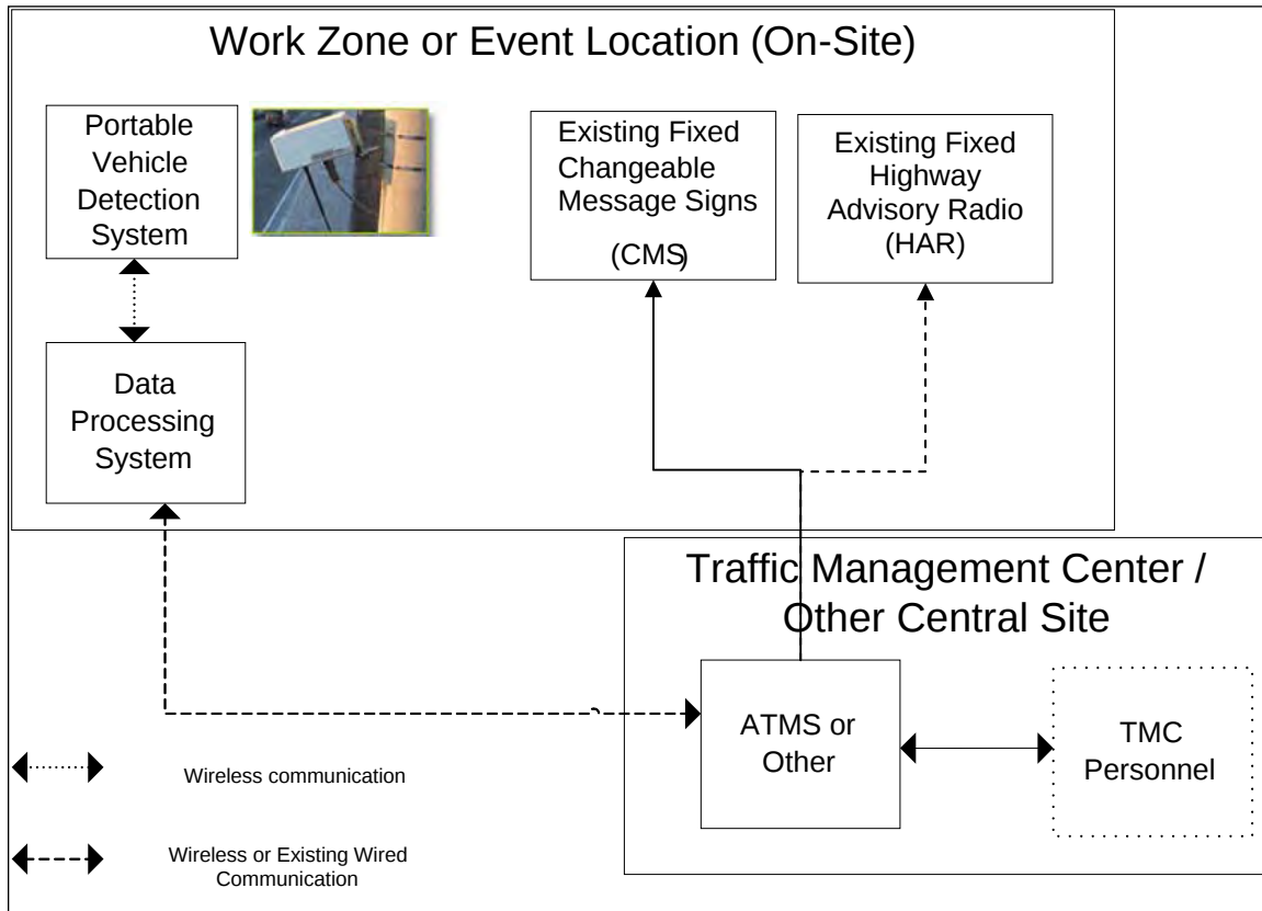
Figure 6. Portable ATIS with Available Fixed CMSs and HARs
