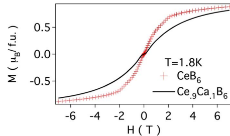
FIG. 6. (Color online) Magnetization per formula unit vs field in \text{CeB}_6 and \text{Ce}_{0.95}\text{Ca}_{0.05}\text{B}_6 .
