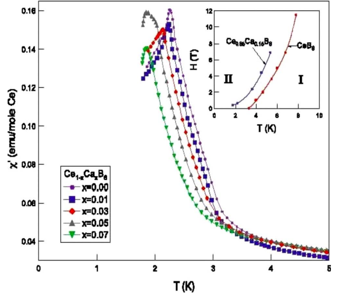
FIG. 5. (Color online) Susceptibility of Ca-doped \text{CeB}_6 , taken at an applied field of 10 Oe showing the suppression of the AFM ordering temperature with increasing x . Inset: Phase diagram for x=0.15 , showing the suppression of the paramagnetic to the AFQ transition temperature, as compared to pure \text{CeB}_6 .
