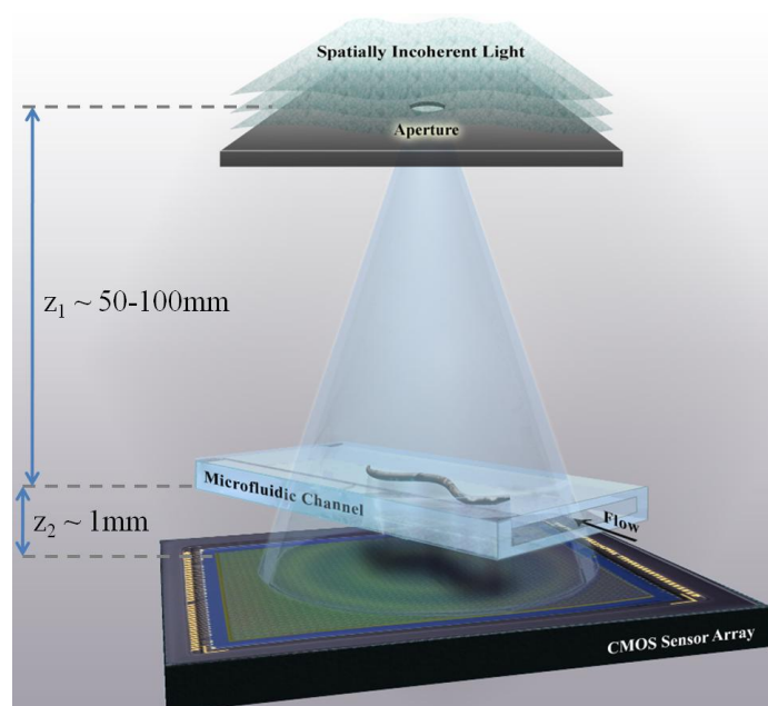
Fig. 1. A schematic of the experimental set-up of Holographic Opto-fluidic Microscopy (HOM). The sample to be imaged flows within a micro-fluidic channel, due to either electro-kinetic or pressure driven motion, and is illuminated by partially coherent light emanating from a large aperture ( \sim 0.05 - 0.1 mm) placed \sim 50 - 100 mm from the sample. The micro-channel is placed directly on a digital sensor array with no additional manipulation of the sensor-chip. (Not to scale.) The propagation distance between the aperture and the sample allows for spatial coherence to develop at the sample plane, and light scattered by the sample interferes with the background light to form a hologram on the sensor array plane.
