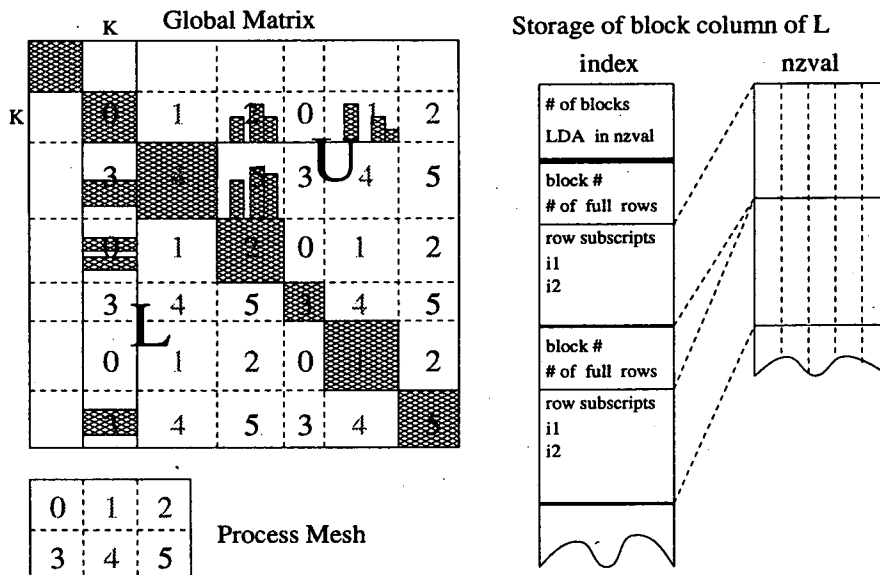
Figure 4.1: The 2-D block-cyclic layout and the data structure to store a local block column of L .
