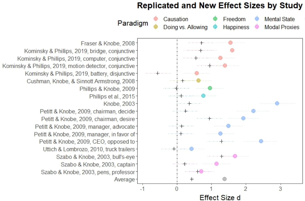
Figure 1: Effect Sizes by Study : Replication effect sizes of the original effects (normal vs. norm-violation) are marked by dots, effect sizes of the new effect (normal vs. ignorant norm-violation) are marked by crosses. Error bars depict 95% confidence intervals of effect sizes
