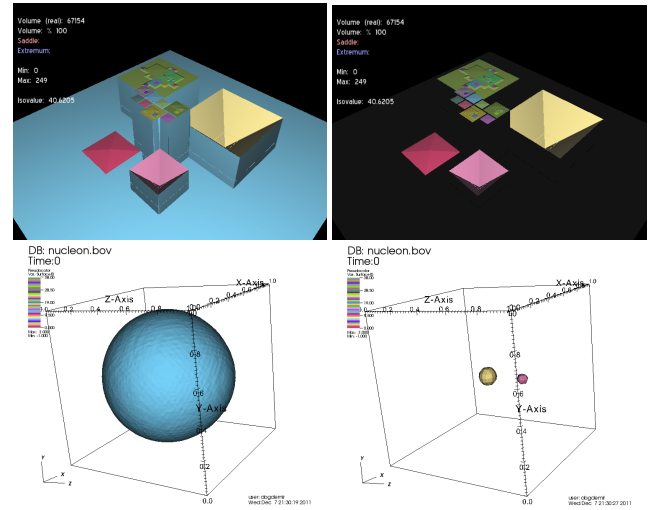
Figure 8: Nucleon data set. (Left) General view of the landscape together with linked isosurface. We see only outer blue component that occludes two inner blobs. (Right) Hiding outer blue component resolves the occlusion.
