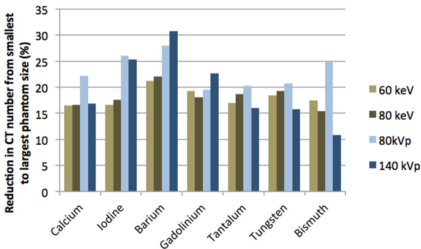
Figure 3. Percentage reduction in CT number from smallest (257 mm effective diameter) to the largest (438 mm effective diameter) phantom size.
