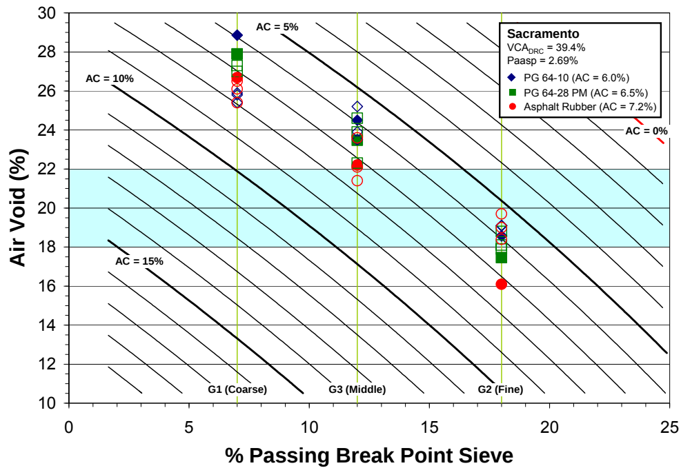
Figure 6.5: OGFC mix design chart calibrated with P_{aasp} = 2.69 percent (Sacramento, Phase I).
