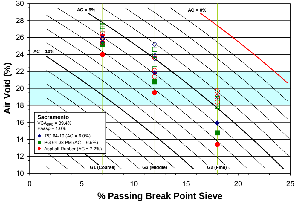
Figure 6.1: OGFC mix design chart (Sacramento, P_{aasp} = 1.0\% ).
