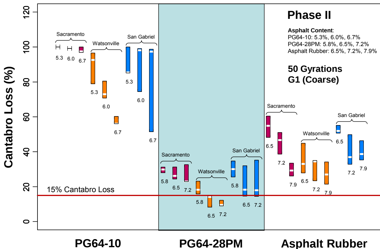
Figure 4.3: Boxplot summary of Cantabro test percent loss results.
