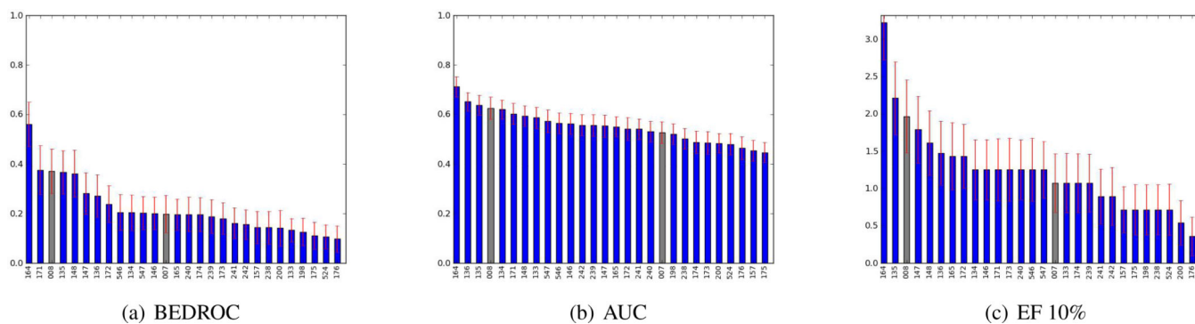
Fig. 2. Calculated metrics for SAMPL4 virtual screening statistics, graphed in ranked order. The statistics are as given in Table 1. Note that many submissions have overlapping error bars, so ranked order is not necessarily indicative of significantly better performance.
