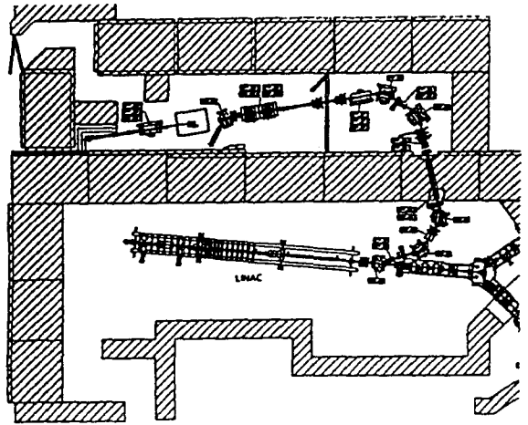
Figure 2: CAD lay-out of the BTF-line
