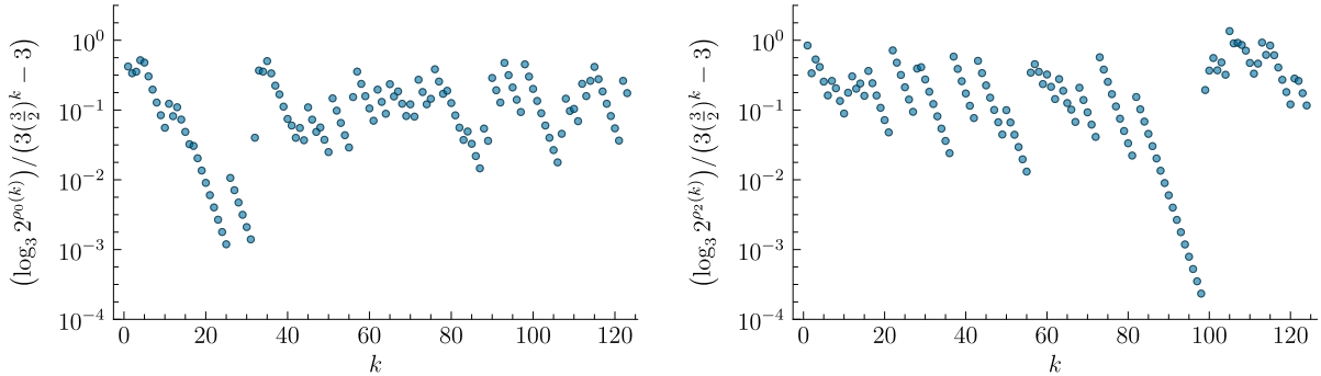
Figure 3: Length of the ternary representation of 2^{\rho_\chi} (being approximately \rho_\chi \log_3 2 ) as a fraction of the expected number of rolls of three-sided die required to generate an uninterrupted sequence of k non- \chi digits (that average roll count being 3(\frac{3}{2})^k - 3 ).
