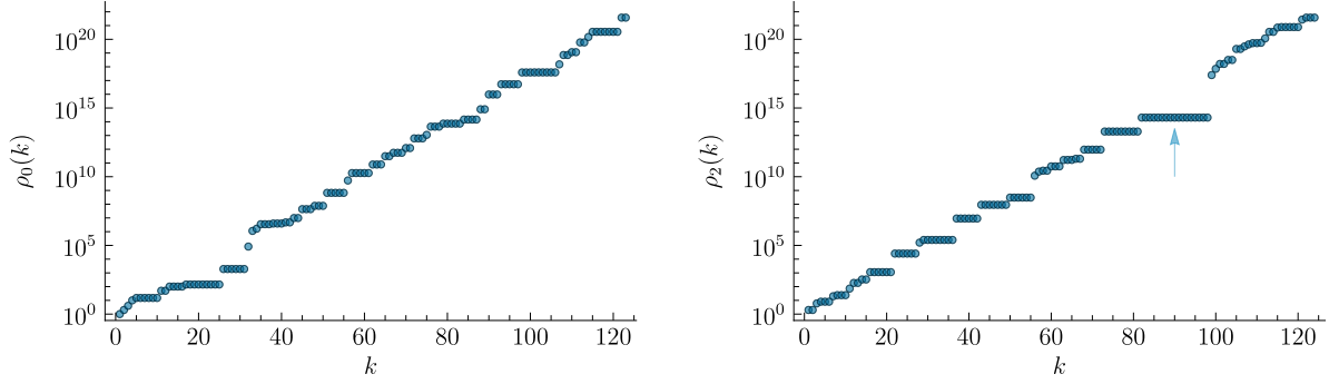
Figure 2: Plots of \rho_0 (resp., \rho_2 ), defined as the smallest integer n such that the digit 0 (resp., 2) occurs nowhere in the last k ternary digits of 2^n . The arrow points to the instance where \rho_2(k) = 201015414581294 for all 82 \leq k \leq 98 .
