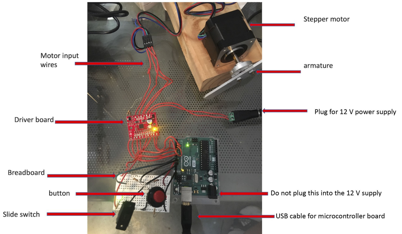
Figure 3: Components of the habituation device. All the labeled electronics are required to assemble the machine.
