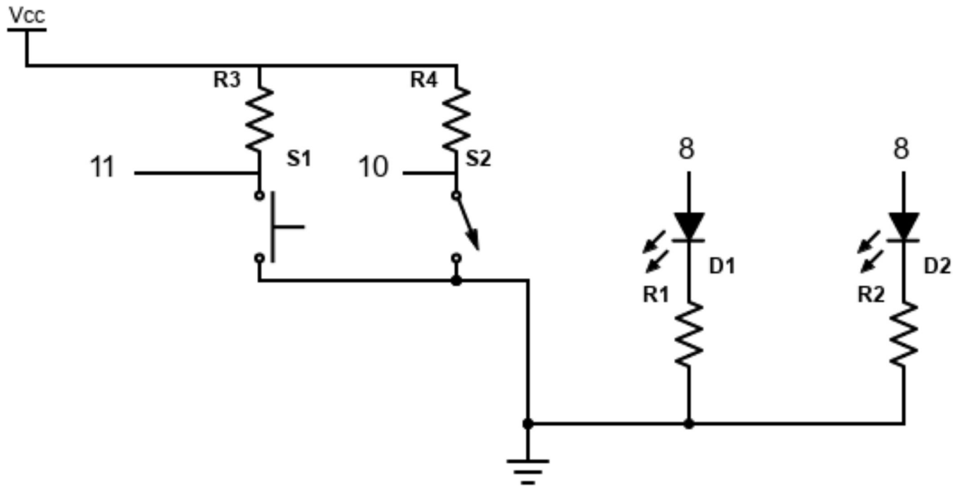
Figure 4: Electronics schematic.
