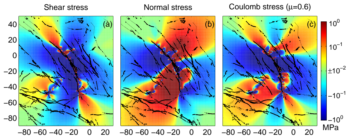
Figure 12. Static stress changes due to the Landers earthquake, in megapascals, on vertical faults striking 35^\circ NW, at depth of 2 km. (a) Shear stress change. (b) Normal stress change. (c) Coulomb stress change. Extensional, and right-lateral shear and Coulomb stress changes are considered to be positive. Coulomb stress changes are computed assuming the coefficient of friction of 0.6. Horizontal coordinates are in km, with origin at the Hector Mine epicenter.
