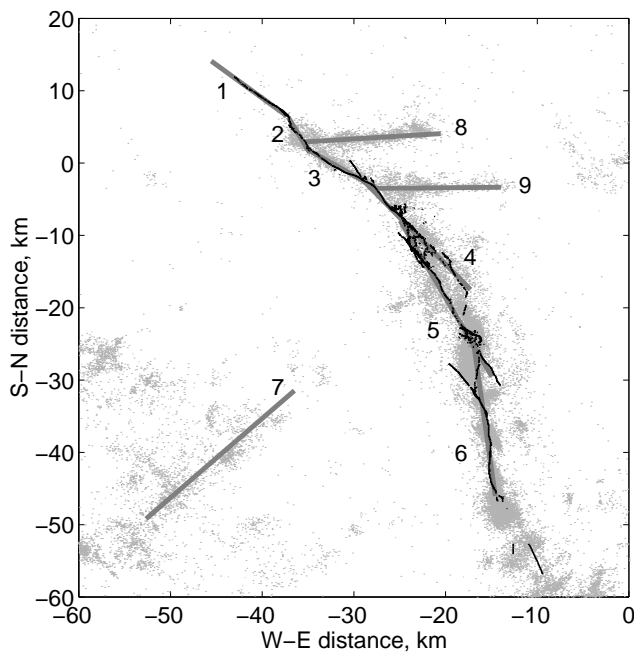
Figure 4. Fault model used to simulate the Landers rupture. Shown are the top edges of the model sub-faults (dark grey lines) superimposed on the mapped fault rupture (black wavy line) and aftershocks (light grey dots).
