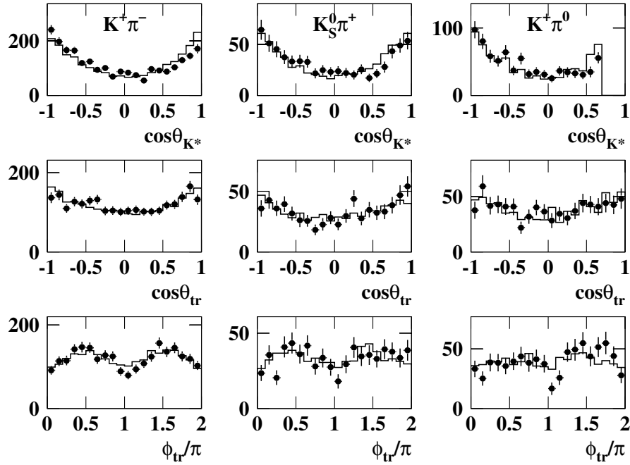
FIG. 4. Angular distributions. Histogram: Inclusive J/\psi MC sample ( p_{J/\psi}^* > 1.3 GeV/ c ). Points: Data. The spectra are acceptance-corrected, background-subtracted, and normalized to the estimated yields (Table II). The visible forward-backward discrepancy in the \cos\theta_{K^*} distribution is due to the K\pi S -wave amplitude present in the data, and absent in the MC sample. The related systematic uncertainties in the measurements of the decay amplitudes are listed in line seven of Table V.
