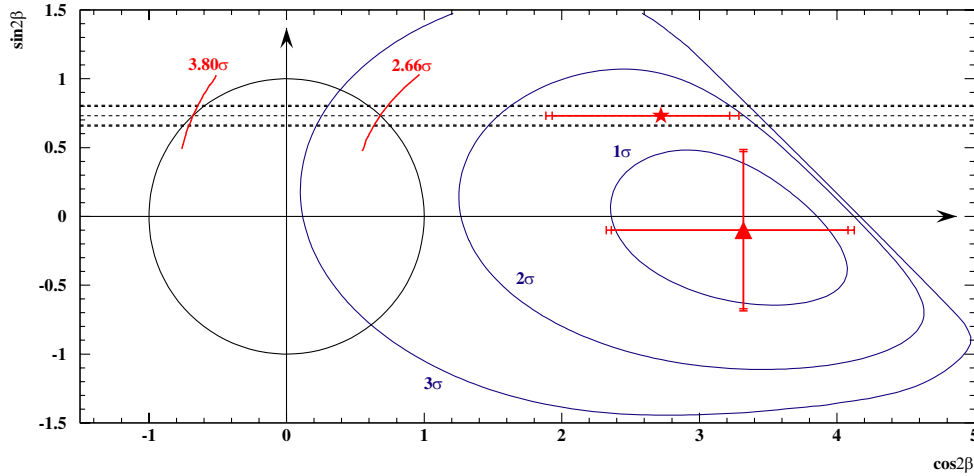
FIG. 10 (color online). Contour plots in the \cos 2\beta , \sin 2\beta plane. The triangle denotes the result of the fit. The error bars show the statistical uncertainty and the quadratic sum of the statistical and systematic uncertainties. The star denotes the result of the fit with \sin 2\beta fixed at \sin 2\beta = 0.731 [4]. The value of \sin 2\beta of Ref. [4] and its uncertainties are represented as dashed horizontal lines. The n\sigma ( n = 1, 2, 3 ) contour corresponds to a decrease of 0.5n^2 in the log-likelihood with respect to the maximum value. The unit circle ( \cos^2 2\beta + \sin^2 2\beta = 1 ) on which the true values must lie is also shown.
