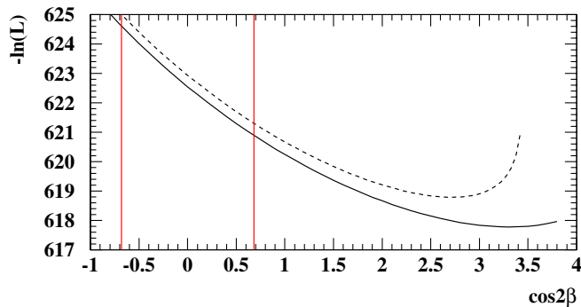
FIG. 13 (color online). The negative logarithm of the likelihood as a function of \cos 2\beta . Continuous line: \sin 2\beta is a free parameter. Dashed line: \sin 2\beta is fixed at \sin 2\beta_0 = 0.731 [4].
