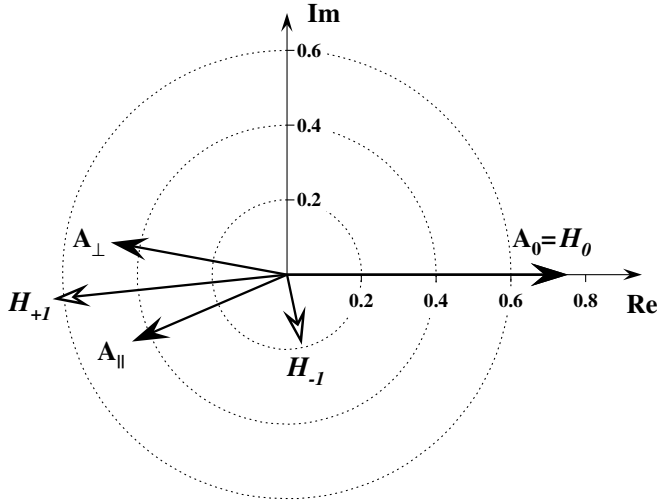
FIG. 16. Representation in the complex plane of the measured transversity amplitudes ( A_0, A_{\parallel}, A_{\perp} ) (Eq. (67)) and the equivalent helicity amplitudes ( H_0, H_{-1}, H_{+1} ) obtained using Eq. (69). The values for H_+ and H_- are quoted in Table XII.
