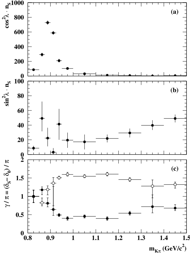
FIG. 7. (a) The P -wave intensity times number of events, i.e., n_S \cos^2 \lambda ; (b) the S -wave intensity times number of events, i.e., n_S \sin^2 \lambda . These are the numbers of events that would be observed in each interval for the amplitude under consideration, if it were the only amplitude. The fraction of S -wave intensity integrated over the range 0.8 < m_{K\pi} < 1.0 \text{GeV}/c^2 is found to be (7.3 \pm 1.8)\% . (c) The evolution of \gamma/\pi with m_{K\pi} , for the two sets of strong phases. The mirror symmetry described by Eq. (10) is clearly visible as \gamma \leftrightarrow 2\pi - \gamma . The error bars represent the statistical uncertainty in the fit of (\lambda, \gamma) in the m_{K\pi} interval considered. All distributions are from fits to J/\psi K^\pm \pi^\mp candidates in data.
