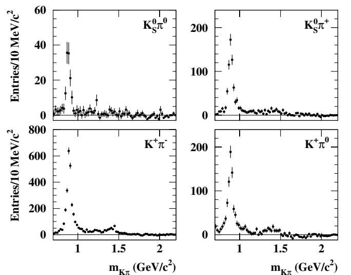
FIG. 5. The background-subtracted K\pi invariant mass distributions for J/\psi K\pi candidates in data.
