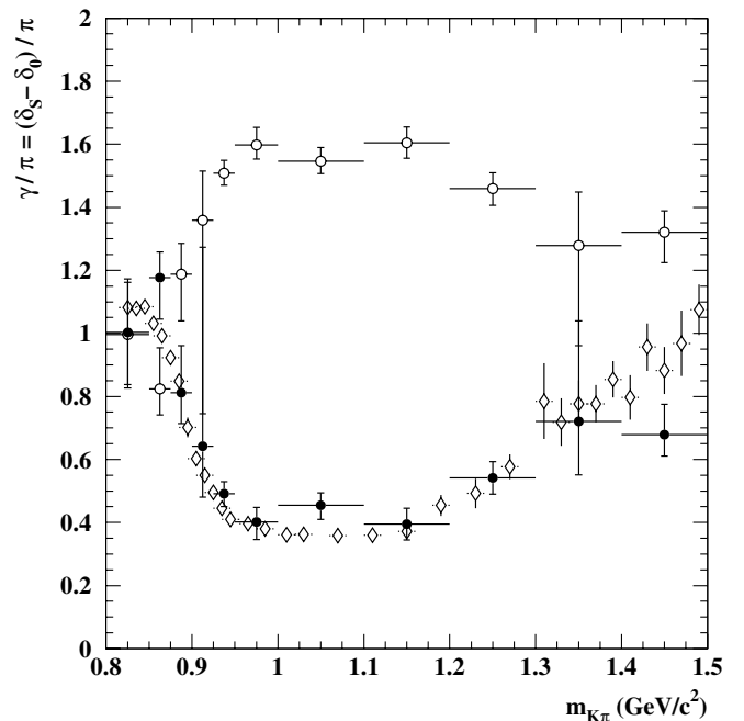
FIG. 9. Comparison of the variation of \gamma = \delta_s - \delta_0 with m_{K\pi} for the J/\psi K^{\pm}\pi^{\mp} events, for “Solution I” (open points, Eq. (28)) and “Solution II” (full points, Eq. (29)), with that measured by the LASS experiment [22,39,40] (diamond markers).
