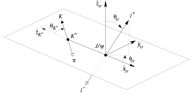
FIG. 1. Definition of the transversity angles ( \theta_{K^*} , \theta_{lr} , \phi_{lr} ) and coordinate system ( \hat{x}_{lr} , \hat{y}_{lr} , \hat{z}_{lr} ). The direction opposite to the B meson momentum in the J/\psi rest frame is \hat{x}_{lr} ; \hat{y}_{lr} is perpendicular to \hat{x}_{lr} in the plane that contains \hat{x}_{lr} and \vec{p}_K , chosen so \vec{p}_K \cdot \hat{y}_{lr} > 0 ; \hat{z}_{lr} = \hat{x}_{lr} \times \hat{y}_{lr} . The helicity angle \theta_{K^*} of the K^* decay is the angle between the direction opposite to the B meson flight direction and the kaon momentum, in the K^* rest frame. Finally, \theta_{lr} and \phi_{lr} are the polar and azimuthal angle of the positive lepton defined in the J/\psi rest frame.
