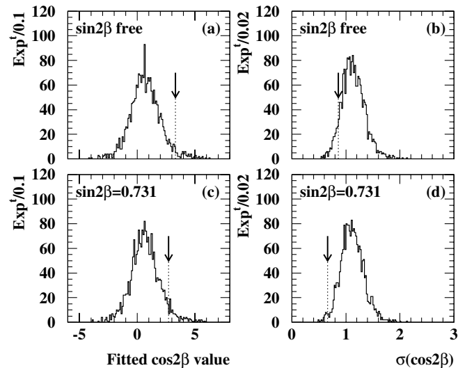
FIG. 14. The distribution of the values of \cos 2\beta ((a) and (c)), and of the statistical uncertainties ((b) and (d)), obtained in 2000 simulated experiments, each based on a sample of the same size as the data; i.e., 104 events. These are taken from the parameterized MC sample mentioned above, with the generated \cos 2\beta value +0.68 . In (a) and (b) \sin 2\beta is also free in the fit. In (c) and (d) \sin 2\beta is fixed to the world average. The vertical arrows show the positions of the values obtained from the data.
