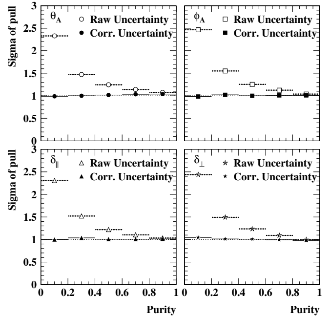
FIG. 17. Root mean square (RMS) of the pull distributions as a function of signal purity (defined in the 5.2 \text{ GeV}/c^2 - 5.3 \text{ GeV}/c^2 m_{ES} range), for the fitted parameters \theta_A , \phi_A , \delta_{\parallel} , and \delta_{\perp} . Open symbols denote the RMS of the pulls computed with the uncertainties taken directly from MINUIT. Closed symbols denote the uncertainties computed according to Eq. (A1).
