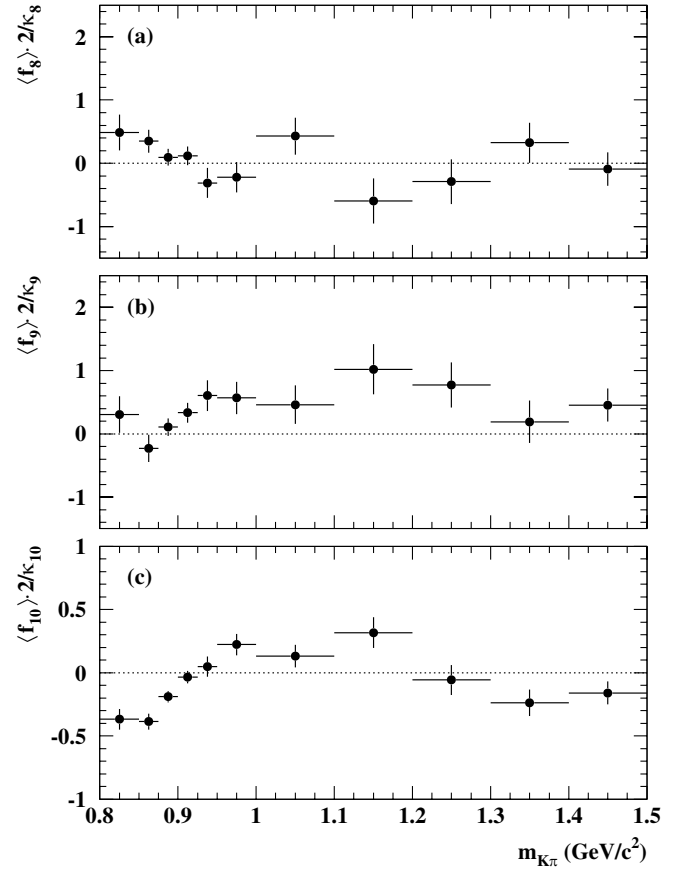
FIG. 6. Measured values of (a) \langle f_8 \rangle \cdot 2/\kappa_8 , (b) \langle f_9 \rangle \cdot 2/\kappa_9 and (c) \langle f_{10} \rangle \cdot 2/\kappa_{10} , defined in Eq. (32), as a function of m_{K\pi} , for the J/\psi K^\pm \pi^\mp candidates in data. The three distributions show a clear variation near the K^*(892) region.
