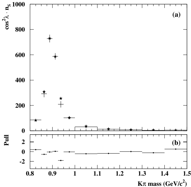
FIG. 8. (a) Comparison of the K^{\pm}\pi^{\mp} P -wave intensity with a Breit-Wigner lineshape, including a centrifugal barrier factor, with world average parameters for K^*(892) [34]. The lineshape is integrated in each mass interval (star markers) and compared with the measured intensity in that interval, after a minimum \chi^2 fit of the overall normalization to the data in the 0.8 \text{ GeV}/c^2 – 1.3 \text{ GeV}/c^2 mass range. The \chi^2 per degree of freedom is 0.86. (b) Pull (i.e. difference of measured and expected intensities, normalized to the uncertainty) in each mass interval.
