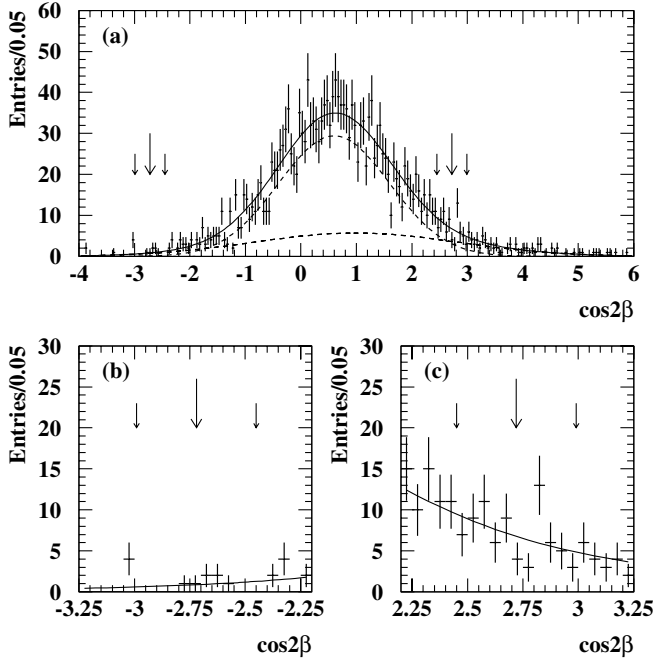
FIG. 15. (a) The \cos 2\beta distribution for 2000 simulated experiments of the same size as the data sample, where the generated values for \sin 2\beta and \cos 2\beta are +0.731 and +0.68 , respectively, [same as Fig. 14(c)]. An unbinned likelihood fit is performed to this distribution, using the sum of two Gaussian functions. The fit result is shown on the plot (full line) with the individual Gaussian contributions (dashed lines). The long vertical arrows show the \cos 2\beta values \pm 2.72 . The small arrows indicate the extent of systematic uncertainties. (b) and (c) zoom on the \cos 2\beta = \pm 2.72 regions of Fig. 15(a). The densities of points at +2.72 and -2.72 are used to discriminate between the \cos 2\beta = \pm \sqrt{1 - \sin^2 2\beta_0} = \pm 0.68 hypotheses, as explained in the text.
