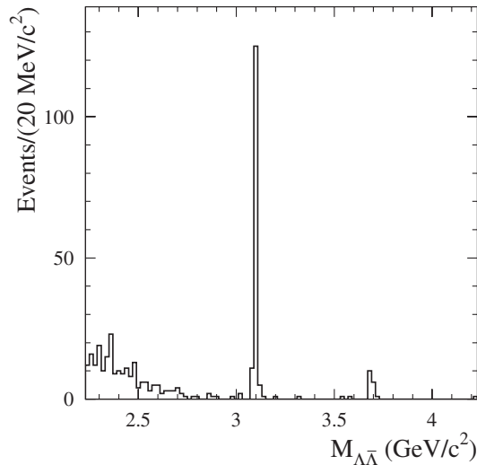
FIG. 4. The \Lambda\bar{\Lambda} mass spectrum for events satisfying the \Lambda\bar{\Lambda}\gamma selection criteria.
