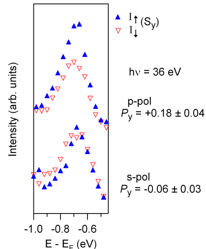
FIG. 5: (Color online). Spin-resolved EDCs of VB peak, taken along k_x ( \Gamma\text{M} ), similar to Fig. 2(b). Spin is measured along \hat{\mathbf{y}} . The upper (lower) EDC is taken with p -polarized ( s -polarized) light with \hat{\boldsymbol{\epsilon}} within the xz -plane ( yz -plane). The reported P_y values for each are integrated through the full energy range shown.
