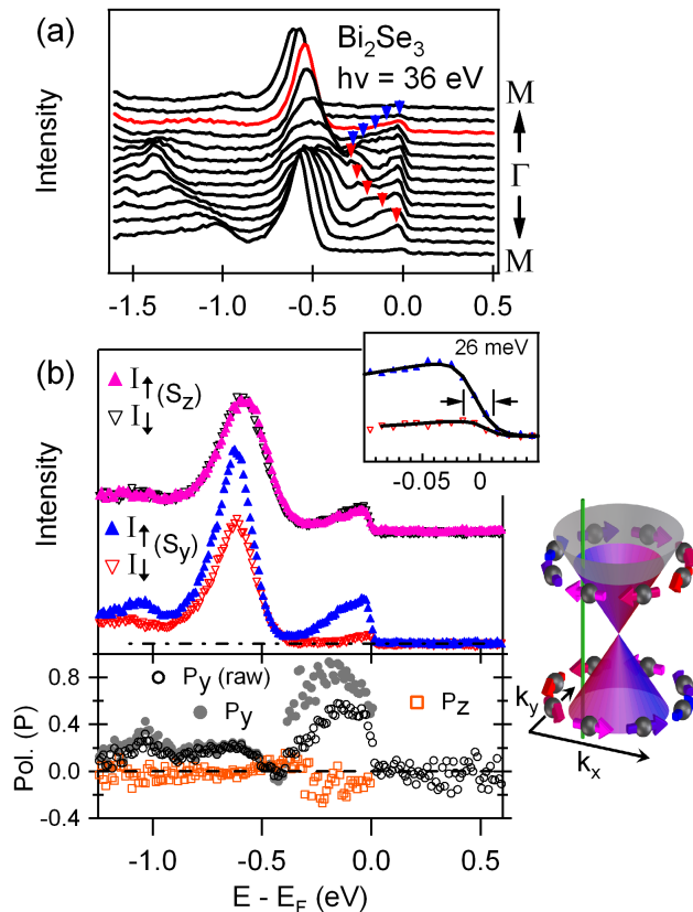
FIG. 2: (Color) (a) Spin-integrated EDCs as a function of momentum along k_x ( \Gamma M ) of \text{Bi}_2\text{Se}_3 . UDC peaks are marked by blue (spin-up) and red (spin-down) arrows according to the predicted P_y . Other peaks are related to bulk bands. (b) Spin-resolved EDCs corresponding to the red EDC in (a), with the spin quantization axis along the out-of-plane \hat{z} direction (upper), and the in-plane \hat{y} direction (lower). The EDC location is depicted by the vertical green line in the TSS cartoon inset, and the green circle in the Fig. 1(d) inset. The corresponding spin polarization curves are shown in the bottom panel. Open black circles are the raw P_y , while the solid gray circles correspond to the effective polarization once a constant background (dash-dot line in upper panel) is removed. Inset shows close-up of spin-resolved Fermi level with Fermi fits.
