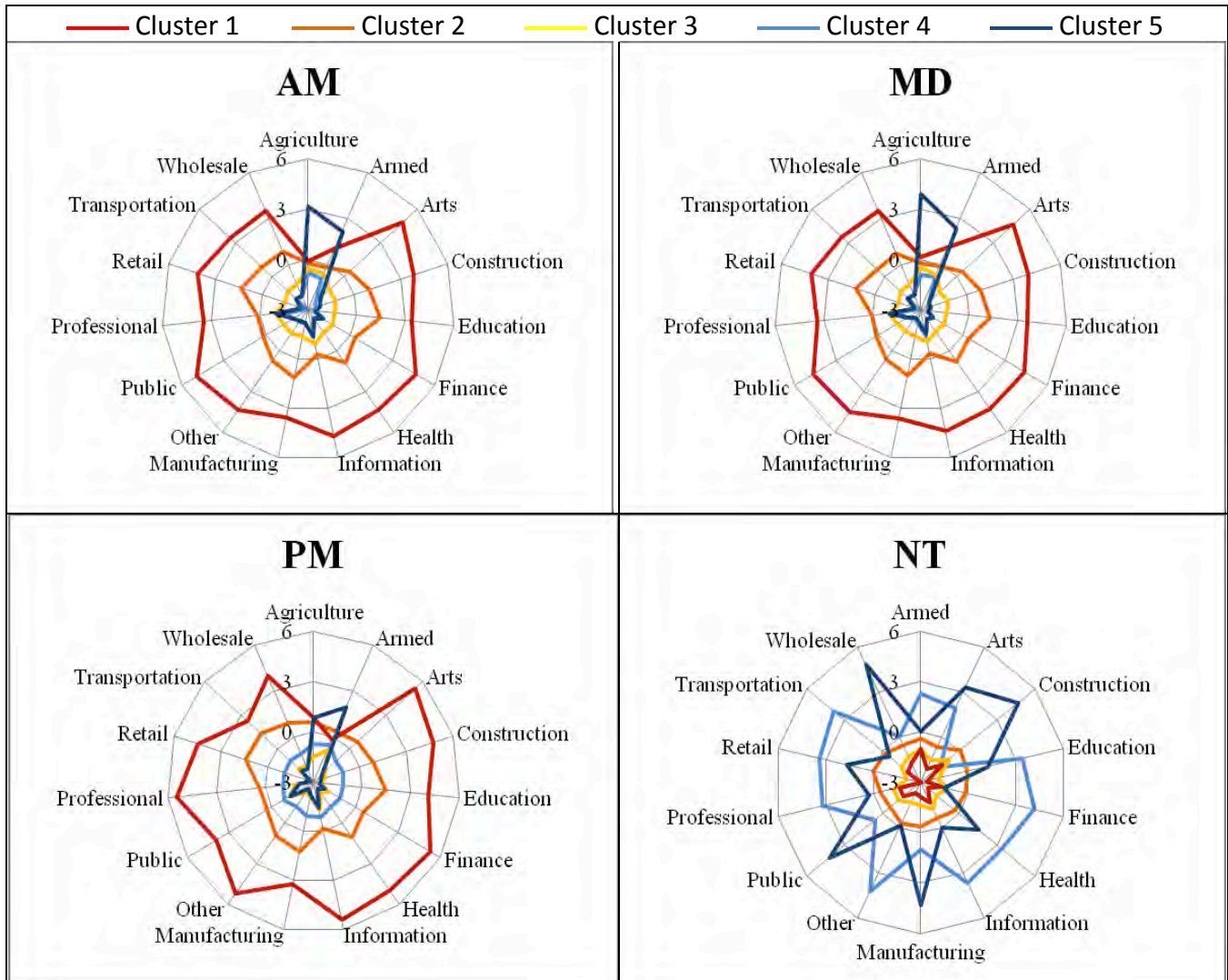
Figure 2 Latent Class Cluster characteristics
