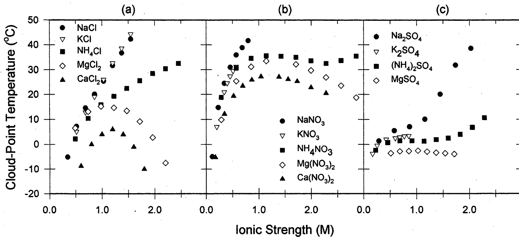
Figure 2. Effect of cations on the cloud-point temperature for lysozyme (87 g/L) at pH 4.0 for (a) Cl - , (b) NO 3 - , (c) SO 4 2- aqueous salt solutions. The trends for pH 4.0 are similar as for pH 7.0
