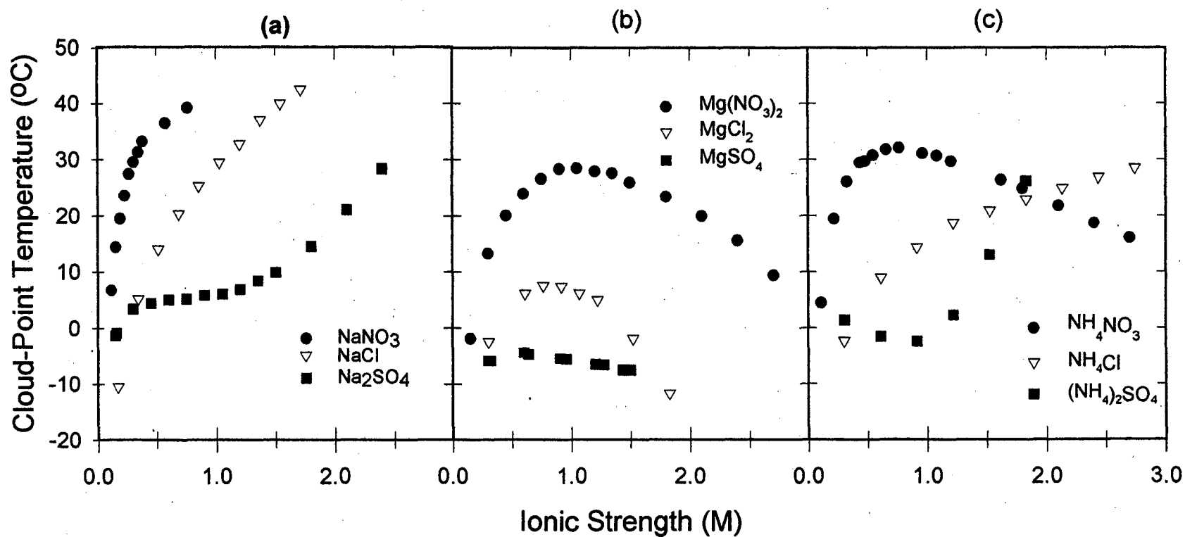
Figure 3. Effect of anions on the cloud-point temperature for lysozyme (87 g/L) at pH 7.0 for (a) Na + , (b) Mg 2+ , (c) NH 4 + aqueous salt solutions. As the anion becomes more kosmotropic, the CPT decreases at a specific salt concentration. While potassium and calcium salts are not included, they follow the same trends as the sodium and magnesium salts, respectively.
