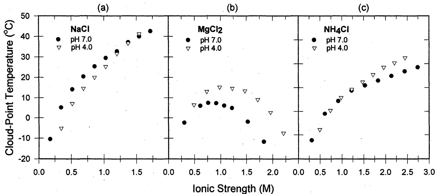
Figure 5. Effect of pH on the cloud-point temperature for lysozyme (87 g/L) for (a) NaCl, (b) MgCl 2 , (c) NH 4 Cl aqueous salt solutions. For NaCl as salt concentration increases, the difference in CPT decreases due to charge-charge screening. For MgCl 2 , as salt concentration increases, the difference in the CPT increases. Greater Mg 2+ binding at pH 4.0 leads to a greater hydration force and hence a lower CPT. The trends for NH 4 Cl is a combination of the charge screening and hydration force effects.
