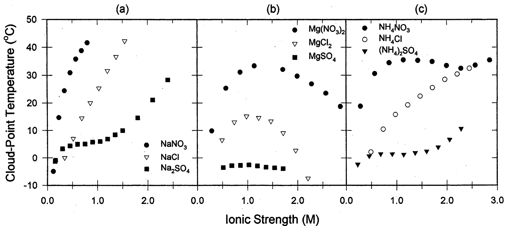
Figure 4. Effect of anions on the cloud-point temperature for lysozyme (87 g/L) at pH 4.0 for (a) Na + , (b) Mg 2+ , (c) NH 4 + aqueous salt solutions. Trends are similar to pH 7.0. Again, the trends for potassium and calcium salts are similar to the sodium and magnesium salts, respectively.
