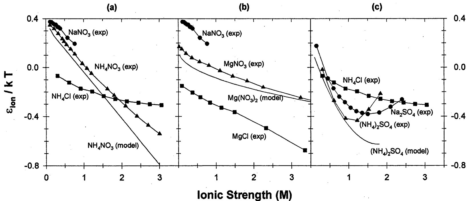
Figure 6. Representative plots of combinations of \epsilon_{ion}/kT for (a) monovalent ions (b) divalent cations and \text{NO}_3^- and (c) monovalent cations with \text{SO}_4^{2-} . It was assumed that \text{Na}^+ and \text{Cl}^- were ideal ions and did not contribute to \epsilon_{ion}/kT of the appropriate counterion. The solid line (no symbols) represents \epsilon_{ion}/kT calculated from the model. Plot (a) shows that addition of \epsilon_{ion}/kT values gives good results. Plot (b) is the average of \epsilon_{ion}/kT since \text{Mg}^{2+} is a solution structure former and \text{NO}_3^- is a structure breaker. Plot (c) shows the addition of \epsilon_{ion}/kT . Model results are in good agreement up to 1M.
