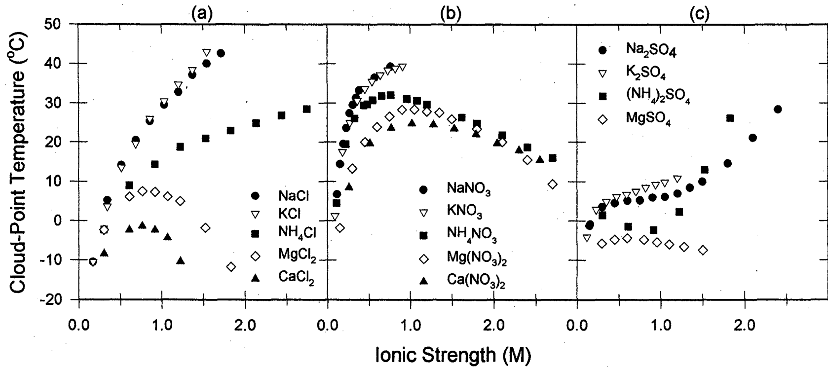
Figure 1. Effect of cations on the cloud-point temperature for lysozyme (87 g/L) at pH 7.0 for (a) Cl - , (b) NO 3 - , (c) SO 4 2- aqueous salt solutions. For different salts, as ionic strength increases the difference in CPT increases, indicating the specific nature of the ions is more important at higher salt concentration. A maximum in the CPT is observed for divalent cationic salts.
