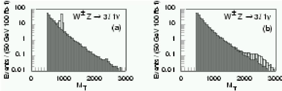
Figure 2: Event yields at the LHC for \rho_T \rightarrow W^\pm Z^0 \rightarrow \ell^\pm \nu_\ell \ell^+ \ell^- for M_{\rho_T} = 1.0, 2.5 TeV; from Ref.[134]. A conventional techni- \rho resonance of mass much above 1 TeV would be invisible in the channel \rho_T \rightarrow W^\pm Z^0 \rightarrow \ell^\pm \nu_\ell \ell^+ \ell^- .
