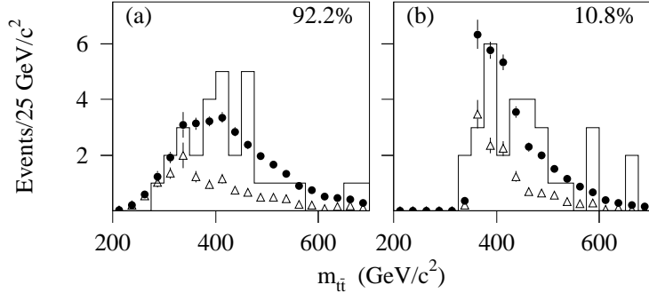
Figure 58: Invariant mass distribution for top pairs: pairs: D0 data (histogram), simulated background (triangles), simulated S+B (dots). In (a) m_t unconstrained; in (b) m_t = 173 GeV.[445–448]
