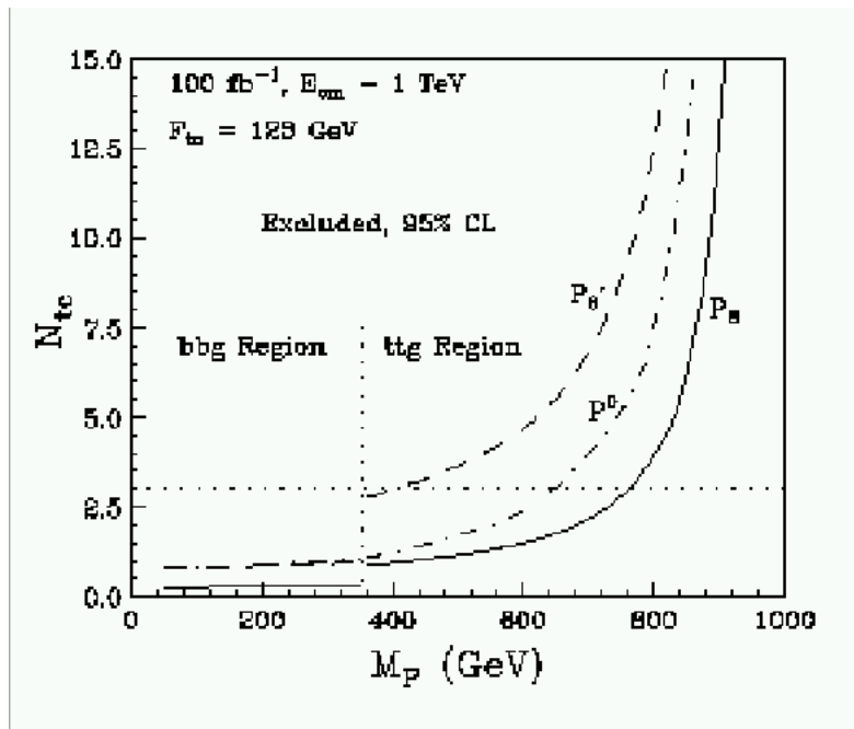
Figure 16: Projected 95% c.l. exclusion reach for electrically neutral PNBs as a function of mass and number of technicolors at a 1 TeV LC [214].
