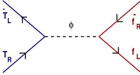
Figure 44: Fermion-technifermion interaction through scalar exchange. This diagram is responsible for fermion mass generation once the technifermions condense.
