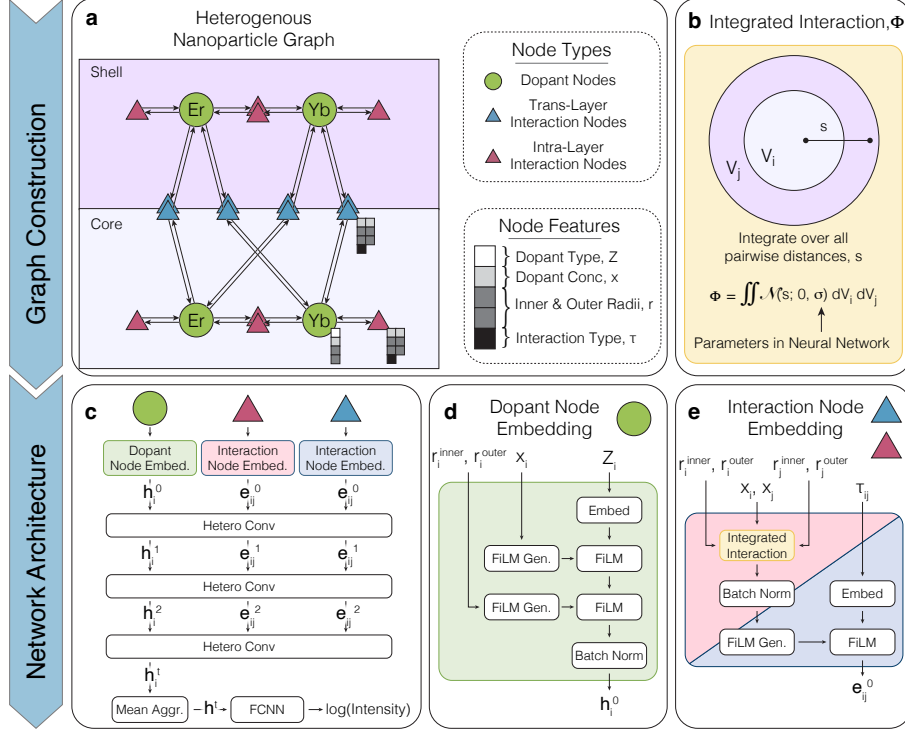
Fig. 3 UCNP graph representation and hetero-GNN model architecture. a) Heterogeneous graph structure of an example two-region (core plus one shell) nanoparticle with Yb and Er dopants. Node types: dopant nodes (green circles), trans-layer interaction nodes (blue triangles), and intra-layer interaction nodes (red triangles). Node features: dopant type Z (atomic number), dopant concentration x (molar fraction), inner radius r^{inner} , outer radius r^{outer} , and interaction type \tau (atomic number of outgoing dopant, atomic number of incoming dopant). b) Depiction of the integrated interaction \Phi between two regions V_i and V_j over all pairwise distances, s , parameterized by learnable parameters, \sigma . Subscripts i and j denote different dopant-region indices. For instance, in (a), Yb in the core, Er in the core, Yb in the shell, and Er in the shell would all have distinct dopant-region indices. c) Architecture of the heterogeneous graph model, showing dopant node embeddings h_i^0 , intra-layer interaction node embeddings e_{ij}^0 , trans-layer interaction node embeddings e_{ij}^1 , and their updates through heterogeneous convolutional layers. The embeddings are combined through mean aggregation into an overall UCNP embedding which is regressed to the \log_{10} of the UV intensity through a fully connected neural network (FCNN). d) Dopant node embedding process, where features r_i^{inner} , r_i^{outer} , x_i , and Z_i form the initial dopant node embedding for dopant-region i , h_i^0 . e) Interaction node embedding process, where features r_i^{inner} , r_i^{outer} , and x_i for dopant-region i , r_j^{inner} , r_j^{outer} , and x_j for dopant-region j , and the interaction type, \tau_{ij} , form the initial interaction node embedding between dopant-regions i and j , e_{ij}^0 .
