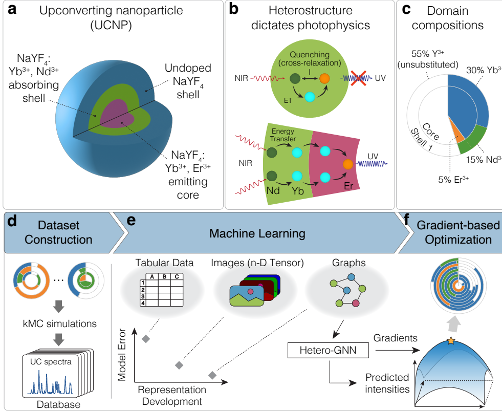
Fig. 1 Deep learning approach to enable UCNP heterostructure optimization. a) Schematic of doping heterostructured UCNPs. b) Illustration of the importance of heterostructuring to physically separate dopants. In the core-only particle, all dopants interact to a high degree, leading to cross-relaxation and consequently low upconversion efficiency, while heterostructuring with Er (orange) and Nd (green) separated into different regions doped with Yb (blue) prevents cross-relaxation and facilitates ultraviolet emission. c) 2D visualization of a heterostructured UCNP with core and shell doping levels for \text{Yb}^{3+} (blue), \text{Nd}^{3+} (green), and \text{Er}^{3+} (orange) represented as colored slices in a concentric pie chart. White regions represent the remaining fraction of \text{Y}^{3+} ions in the \text{NaYF}_4 host matrix that have not been substituted by dopant ions. d) To enable physics-informed deep learning for the inverse design of UCNPs, we first construct a large dataset of simulated UCNPs using high-throughput kMC simulations. e) Then, we investigate different representations of heterostructured UCNPs and find best performance with a heterogeneous graph representation in a GNN. f) The resulting trained model can predict the gradient of emission intensity with respect to each structural parameter, enabling inverse design via gradient-based optimization of UCNP heterostructure to maximize ultraviolet emission.
