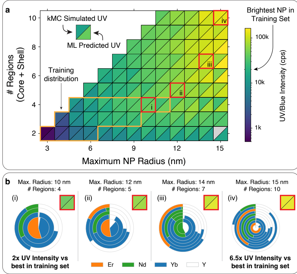
Fig. 5 Gradient-based optimization of UCNPs heterostructure. a) The optimization matrix illustrates I_{vis-UV} intensity (cps) predictions for different particle sizes and numbers of layers. Each square represents the total UV and near-UV intensity obtained from validation (upper left triangle) and predicted by the ensemble of models (lower right triangle). The orange outline encapsulates UCNPs with maximum NP radii and # regions within the training distribution. Red boxes indicate optimized UCNPs that were selected for visualization. See Supplementary Figure 10 for alternate color scheme provided for accessibility. b) 2D visualizations of 4 representative optimized UCNPs from the optimization matrix. The brightest structure, UCNPs (iv), has a UV intensity 6.5x brighter than the brightest UCNPs in the SUNSET-1 training set. Er (orange), Nd (green), Yb (blue), and Y (white) are represented by their respective colors in the 2D visualizations. Note: kMC simulations of the optimized 2-layer 15 nm particle were not possible due to the large number of \text{Er}^{3+} dopants.
