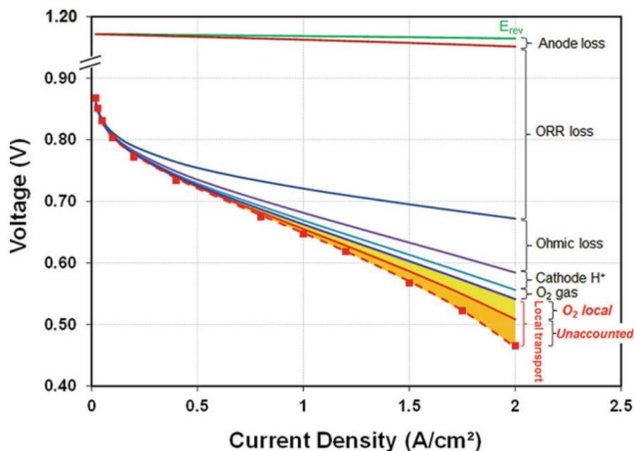
Figure 1-4: Polarization curve of low-Pt loaded PEFC showing voltage loss terms in a low-Pt PEMFC operated under differential cell conditions operated at H 2 /air, 150 kPa, 80°C, and 100% RH. The symbols represent the experimental data. Reprinted with permission from Springer Nature Kongkanand et al., 19 Copyright 2018.
