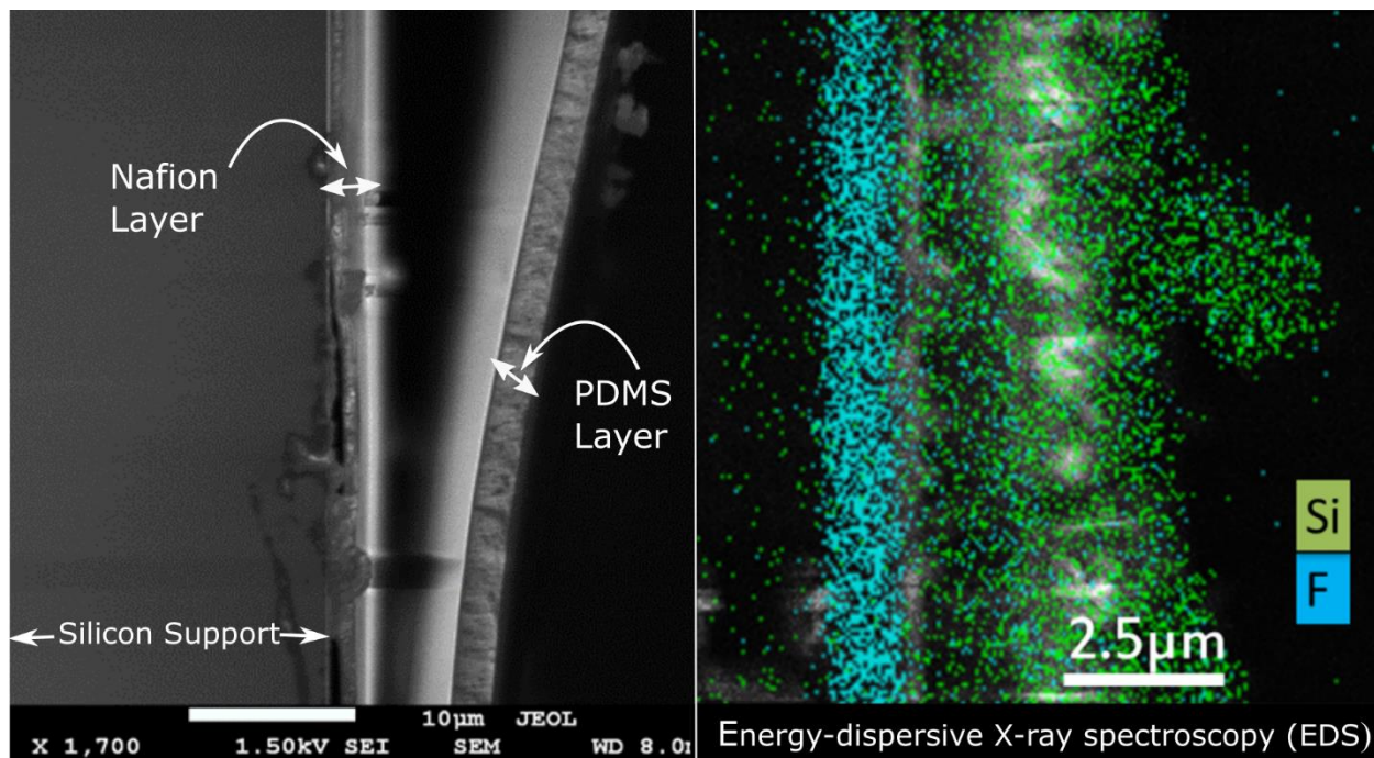
Figure 5-9: (a) Cross-sectional SEM Image of \sim 5\mu\text{m} composite film. (b) Energy-dispersive X-ray spectroscopy (EDS) chemical analysis of cross section of the composite film.
