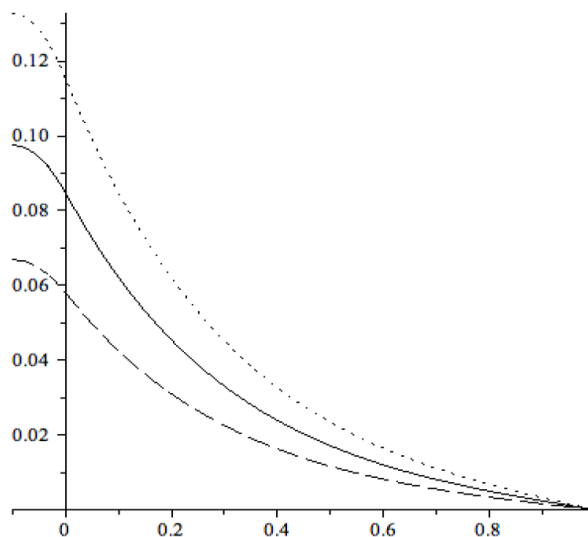
FIGURE 4. Steady state signaling gradients from [12]
