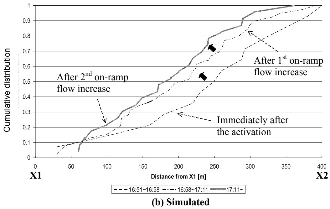
Figure 28. Comparison of cumulative distributions of R-F vehicles' lane changes from 5 to 4 after 16:51 hrs, SR-55N
