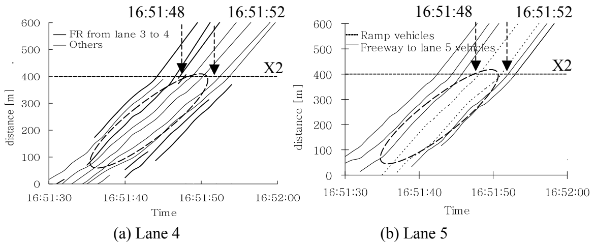
Figure 7. Vehicle Trajectories during period (iii) , SR-55N
