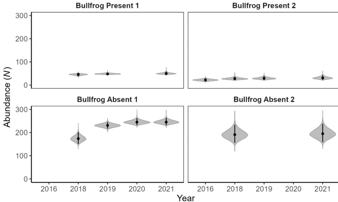
Fig. 2. Annual abundance estimates for Northwestern pond turtles ( Actinemys marmorata ) captured in turtle traps by site and year for sites with (upper panels) and without (lower panels) American bullfrogs ( Rana catesbeiana ). Bullfrog removal occurred from 2016 to 2022 at Bullfrog Present 1 and 2. Points represent posterior medians, vertical lines represent 95 % equal-tailed intervals, and shapes represent posterior distributions.
