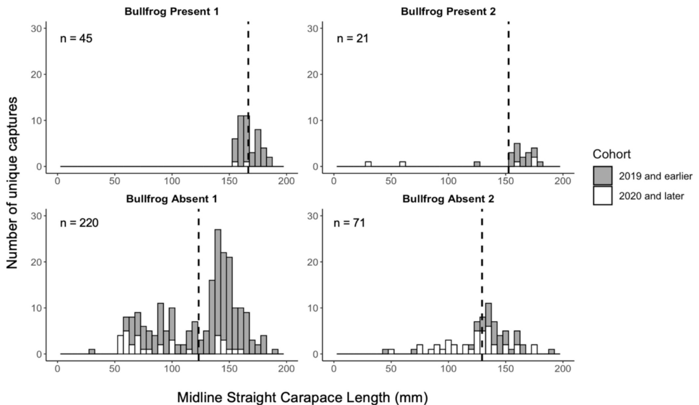
Fig. 3. Size frequency histograms of Northwestern pond turtles ( Actinemys marmorata ) upon first capture. American bullfrog removal occurred at Bullfrog Present 1 and 2 from 2016 to 2022. Bullfrog Absent 1 and 2 had no bullfrog presence. Gray bars represent pond turtles captured in 2019 or earlier, and white bars represent pond turtles captured in 2020 and later after reaching near complete bullfrog eradication. Vertical black dashed lines depict the mean midline straight carapace length for each site across all years. Sample size of individual pond turtles is in the upper left corner of each site's panel.
