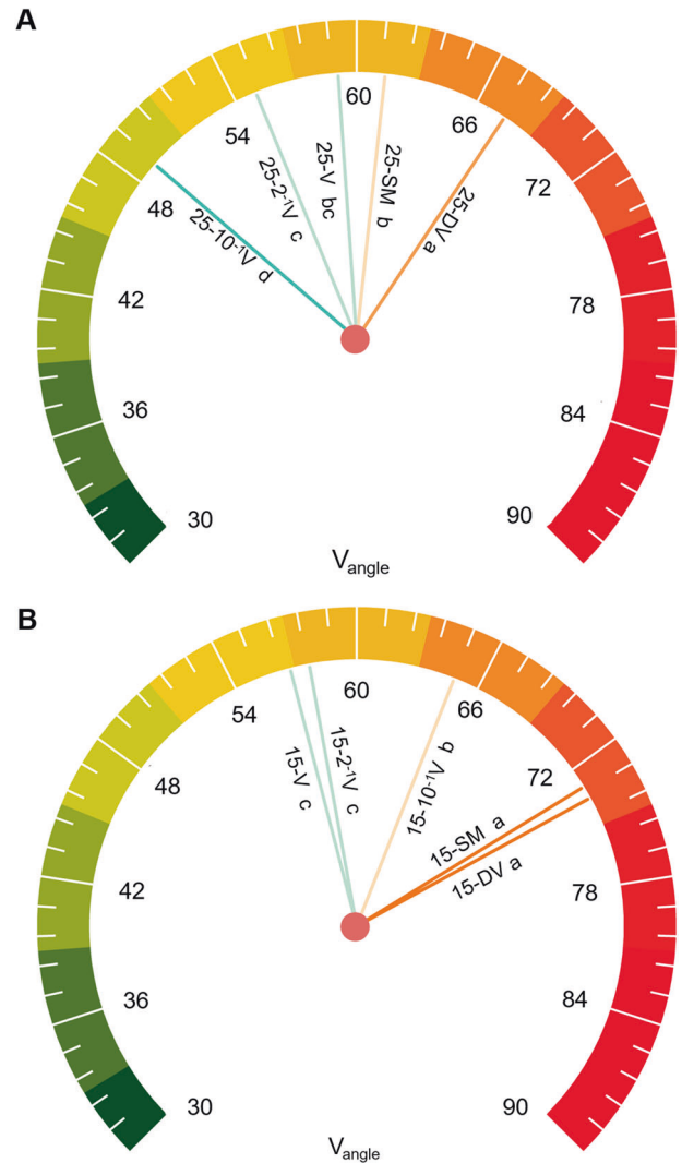
Fig. 3 Microbial resource acquisition strategies. 25°C (A) and 15°C (B). V_{\text{angle}} quantifies the relative P vs. N-acquiring enzyme activities; higher V_{\text{angle}} represents relatively higher P vs. N acquisition strategies. SM, no added viruses; DV, inactive viruses; V, active viruses with no dilution; 2 -1 V, active viruses with twofold dilution; 10 -1 V, active viruses with tenfold dilution; 25 and 15 signify different temperatures (25°C and 15°C) during the incubation. Different lowercase letters represent significant differences at p < 0.05 .
