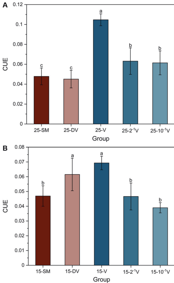
Fig. 2 Carbon use efficiency (CUE) (mean \pm std dev). 25°C (A) and 15°C (B). SM, no added viruses; DV, inactive viruses; V, active viruses with no dilution; 2 -1 V, active viruses with twofold dilution; 10 -1 V, active viruses with tenfold dilution; 25 and 15 signify different temperatures (25°C and 15°C) during the incubation. Different lowercase letters represent significant differences at p < 0.05 .
