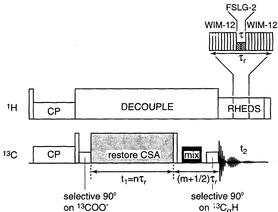
Figure 2.13: The relayed anisotropy correlation (RACO) experiment. This experiment is performed under MAS. After cross-polarization, ^{13}\text{C} magnetization is returned to the z-direction and a selective 90^\circ pulse returns only the ^{13}\text{COO}^- magnetization to the x-y plane. A 6\pi -pulse sequence is used to restore the CSA on this ^{13}\text{COO}^- magnetization for t_1 . During the subsequent mixing period, magnetization exchange between the ^{13}\text{COO}^- and the ^{13}\text{C}_\alpha\text{H} is driven by scaling their chemical-shift difference, with frequency-switched off-resonance irradiation, to match the rotational-resonance condition. A selective 90^\circ pulse on the ^{13}\text{C}_\alpha\text{H} returns its magnetization to the transverse plane. The RHEDS sequence is used during detection so that only the ^{13}\text{C}_\alpha\text{H} - ^1\text{H} dipolar coupling is observed. The entire experiment must be synchronized with rotor cycles, as shown.
