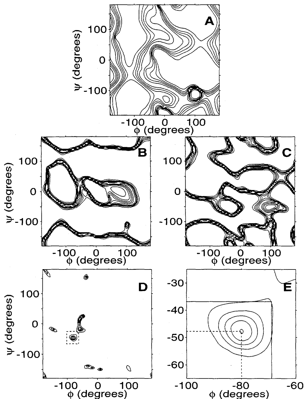
Figure 4.4: Z-surfaces calculated from the experimentally determined chemical-shift anisotropy for the C_\alpha alanine in G*AV and theoretical chemical-shielding surfaces scaled by the correlation determined using A*AA and A*AA-hemihydrate. A. ^1Z -surface for the isotropic shift. B. ^1Z -surface for the width of the CSA ( \delta_{33} - \delta_{11} ). C. ^1Z -surface for the breadth of the CSA ( \delta_{22} - \delta_{11} ). D. ^3Z -surface showing the intersection of the surfaces from A, B, and C. The boxed region contains the area of highest probability and is expanded in E. The dihedral angles as determined by measurement of the CSA tensor are \phi = -79.9^\circ , \psi = -47.8^\circ (dashed lines), while those determined in the crystal structure are \phi = -68.7^\circ , \psi = -38.1^\circ (solid lines). In all cases, contours are plotted at 10%, 30%, 50%, 70%, and 90% of the maximum intensity.
