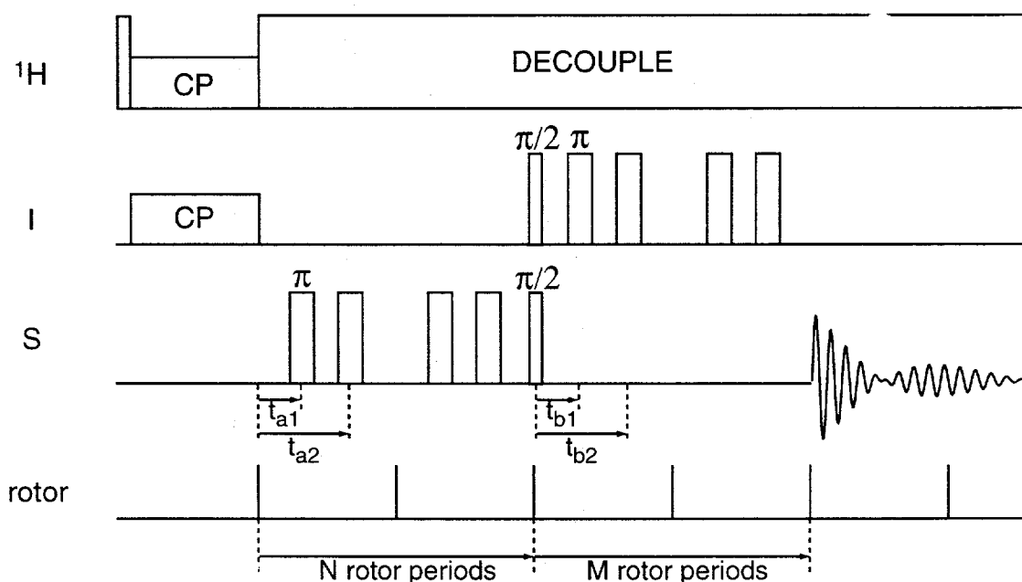
Figure 2.8: The transferred-echo double-resonance (TEDOR) experiment. The entire experiment takes place under MAS. Protons are used for cross-polarization and then decoupled for the remainder of the experiment. After gaining magnetization from protons, I spins evolve for N rotor periods under the influence of two \pi -pulses per rotor cycle on the S spin channel. Simultaneous \pi/2 -pulses on the I and S spins transfer magnetization from I spins to S spins. This magnetization then evolves for M rotor period under the influence of two \pi -pulses per rotor cycle on the I spin channel, after which it is detected. The \pi -pulses are placed at times t_{x1} and t_{x2} , typically at \tau_r/4 and 3\tau_r/4 .
