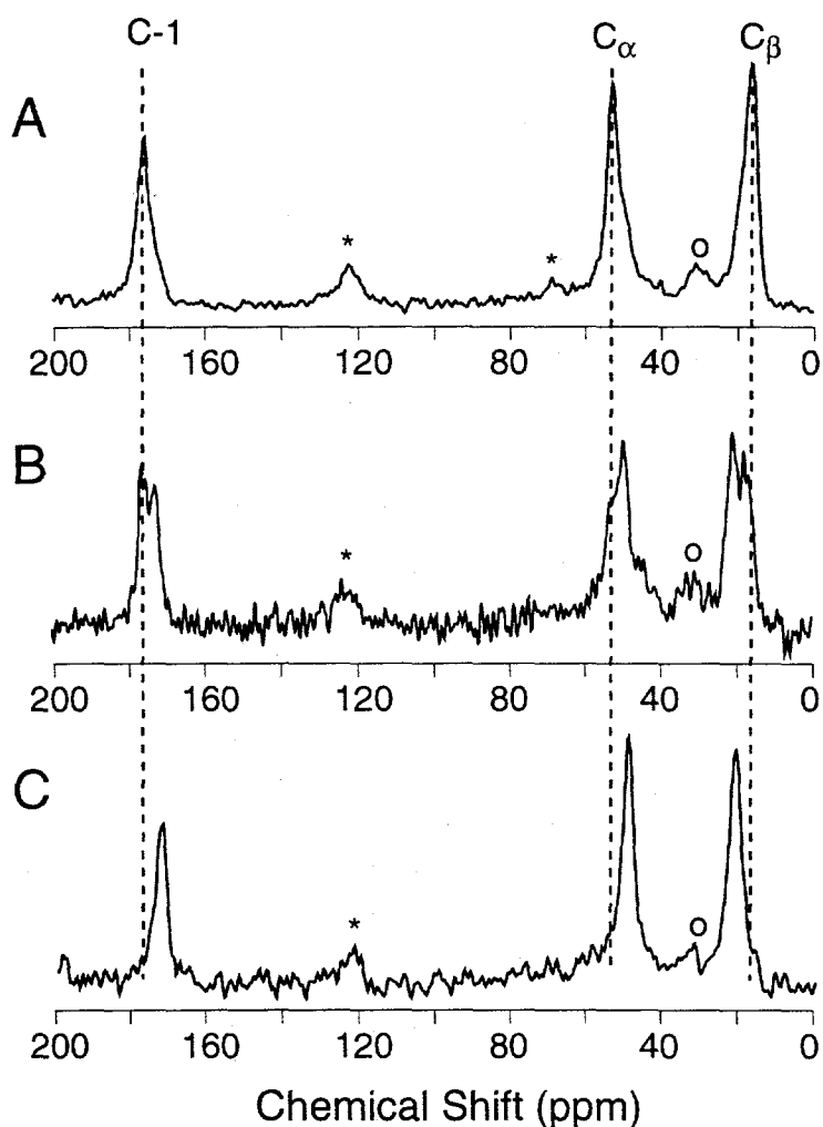
Figure 6.3: CPMAS spectra of a mixture of alanine 115 ^{13}\text{C}=\text{O} , ^{13}\text{C}_{\alpha} , and ^{13}\text{CH}_3 H1 peptides a) lyophilized from HFIP; b) after exposure to air at 30% humidity ( \text{H}_2\text{O} vapor over a saturated solution of \text{CaSO}_4 at 25^\circ\text{C} ) for 30 minutes; c) after 2 hour exposure to air at 100% humidity. Experimental parameters are as in figure 1, except the number of scans were 1024 for A, 2384 for B, and 512 for C, and less sample was used. Peaks marked with a '*' are spinning sidebands and those marked with an 'o' are due to natural-abundance background ^{13}\text{C} . The dotted lines indicate the positions of the shifts when lyophilized from HFIP.
