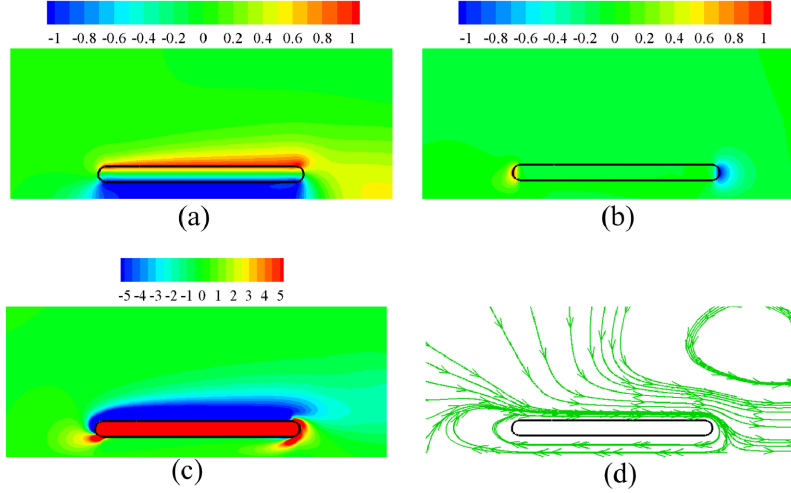
FIG. 9. Near-body flow field around a tethered swimmer visualized through (a) contour of u_x , (b) contour of u_r , (c) contour of vorticity, and (d) streamlines. R_e = 200 , D = 0.3 .
