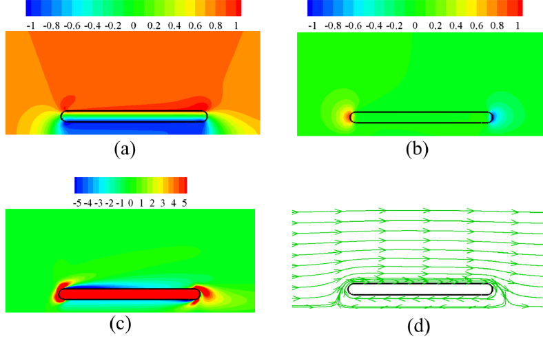
FIG. 15. Near-body flow field around a free-swimming swimmer visualized through (a) contour of u_x , (b) contour of u_r , (c) contour of vorticity, and (d) streamlines. Re = 200 , D = 0.3 . The flow field is recorded in a body-fixed coordinate system.
