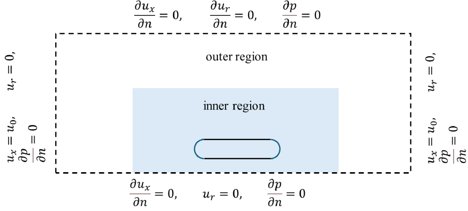
FIG. 4. The computational domain and boundary conditions.
