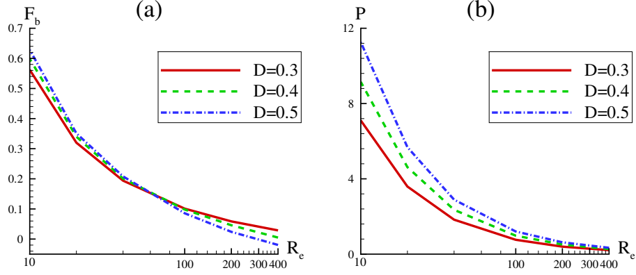
FIG. 12. (a) Net force F_b and (b) power expenditure P in steady state at different values of R_e and D in the tethered mode.
