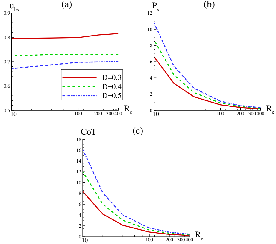
FIG. 14. (a) Swimming speed u_{bs} , (b) power expenditure P_s , and (c) CoT in steady state at different values of R_e and D in the free-swimming mode. The swimming direction is -x (see Fig. 3).
