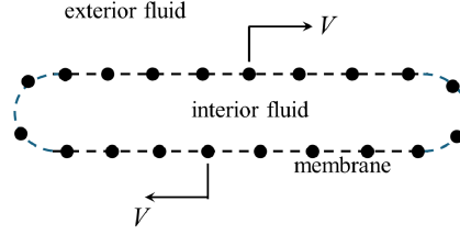
FIG. 5. Numerical rendition of the membrane circulation. The contour of the wall is shown in dashed line, and the numerical grids on the membrane are shown as bullets.
