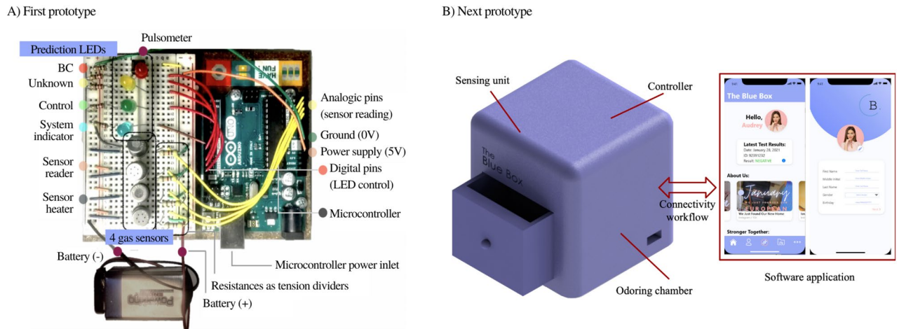
Figure 9. (A) First prototype: Main electronic components that integrate the first eNose prototype. The 4 gas sensors sniff the sample and send a VOC-dependent 0–5 V signal to the Arduinos analogic pins. Their combined signal is then reduced in dimensionality and undergoes sample classification. Depending on the prediction, output digital pins supply current to the corresponding LED, alerting of “possibly BC” “prediction no strong enough”(Blank) or “possibly control”(CTR). (B) Final prototype: Structure of the device and software application that we mentioned above. The 3D-printed structure contains all parts involved in the urine analysis. The software application is the interface to trigger the analysis and receive the results.
