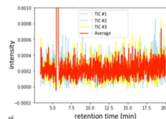
Figure 3. Summary of the pre-processing steps from GC-MS raw data reading up to total ion chromatogram (TIC) design. Sample 151 (belonging to a breast cancer subject) has been used to illustrate those steps.
