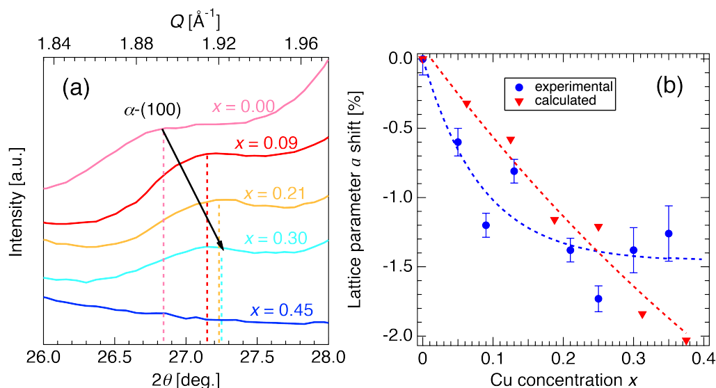
Figure 3. (a) A subset of Figure 1, illustrating a shift of the \alpha -ZnS (100) crystal peak to higher Q for 5 representative films. Dotted lines correspond to peak centers, as determined by a fit to a Voigt and linear background subtraction. (b) The corresponding lattice constant a as a function of Cu concentration (blue circles). Error bars are the standard deviation of the Voigt fit. Red triangles are the expected theoretical lattice shifts for complete Cu substitution from ab initio calculations (see SI). Dashed lines are guides for the eye.
