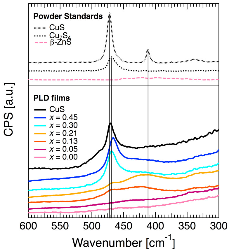
Figure 4. Micro-Raman spectra obtained from \text{Cu}_x\text{Zn}_{1-x}\text{S} films. Raman powder standards of crystalline phases of \text{Cu}_v\text{S} and \text{ZnS} are from the RRUFF project. [48] It should be noted that within a given film, the spectra had a large dependence on lateral position and peaks were not always observed (see text).
