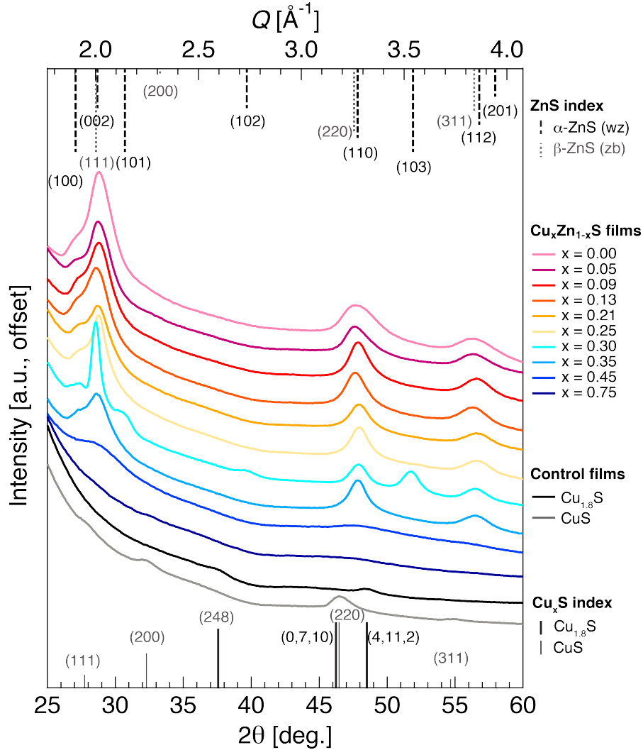
Figure 1. Wide angle X-ray scattering (WAXS) diffraction patterns of \text{Cu}_x\text{Zn}_{1-x}\text{S} films deposited on quartz at room temperature for 0 \leq x \leq 0.75 . Spectra are plotted vs. Q (upper x-axis) and against the equivalent \text{Cu K}\alpha 2\theta diffraction angle (lower x-axis). Films contain a mix of wurtzite (wz, \alpha ) and zinc-blende (zb, \beta ) ZnS. Vertical lines correspond to diffraction standards of the indicated crystal phases from the ICDD powder diffraction database. [59] The control films from the zinc-less targets are nanocrystalline \text{Cu}_{1.8}\text{S} (black trace, from \text{Cu}_2\text{S} target) and \text{CuS} (grey trace, from \text{CuS} target), but no copper sulfide peaks are observed in the \text{Cu}_x\text{Zn}_{1-x}\text{S} films. The background signal is from the quartz substrate.
