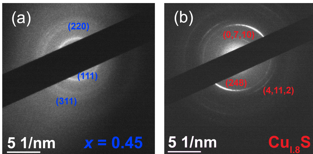
Figure 2. Selected area electron diffraction (SAED) patterns of (a) a \text{Cu}_x\text{Zn}_{1-x}\text{S} film with x = 0.45 . The observed rings are assigned in the figure to the (111), (220), and (311) from \beta -ZnS, but could also be from the closely overlapping \alpha peaks (see Figure 1). (b) SAED pattern from a \text{Cu}_{1.8}\text{S} control film with the indicated indexing. No crystalline Cu-containing phases were observed from the x = 0.45 film shown in (a).
