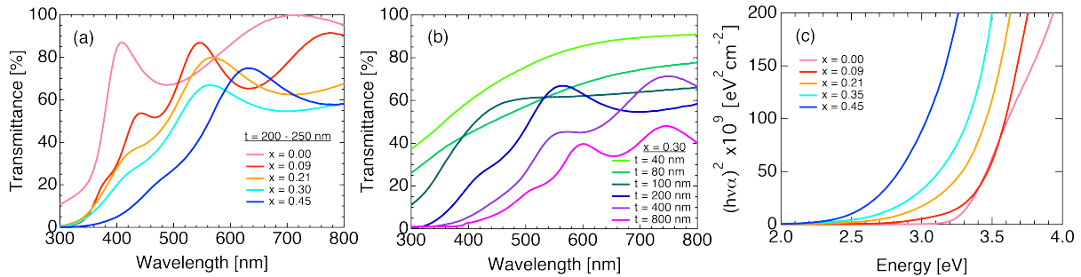
Figure 7. (a) Transmittance as a function of Cu concentration ( x ) and (b) transmittance as a function of film thickness ( t ), both normalized to remove the average absorbance from the quartz substrate. Fringes are due to reflectance from the quartz and air interfaces. (c) Tauc plots derived from ellipsometric measurements of the absorption coefficient are used to estimate the optical band gap as a function of x . Optical band gaps in room temperature deposited films are shown to vary from \sim 2.5 - 3.3 eV.
