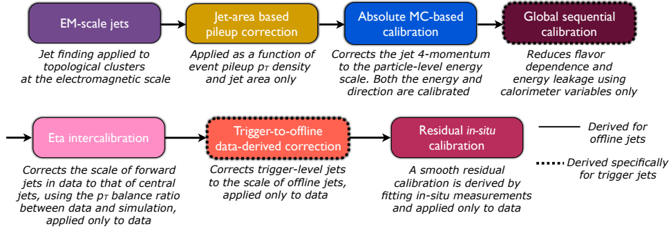
Figure 2: Calibration stages for EM-scale trigger-level jets, each applied to the four-momentum of the jet. MC refers to the simulation.
