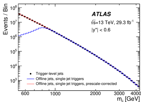
Figure 1: Comparison between the number of dijet events in the data used by this analysis (black points), the number of events selected by any single-jet trigger (thicker, blue line), and the events selected by single-jet triggers but corrected for the trigger prescale factors (thinner, red line) as a function of the dijet invariant mass ( m_{jj} ). The definition of y^* is (y_1 - y_2)/2 , where y_1 and y_2 are the rapidities of the highest- and second-highest- p_T jets.
