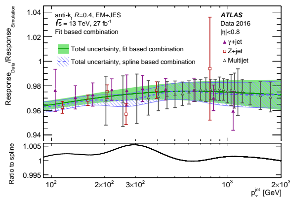
Figure 3: The in situ calibration in the range 85 \text{ GeV} < \text{jet } p_T < 2 \text{ TeV} , for both the spline (dashed line) and fitted (solid line) combination methods, as described in the text. Data points from the three input measurements are overlaid. The lower panel shows the ratio of the two calibration curves.
