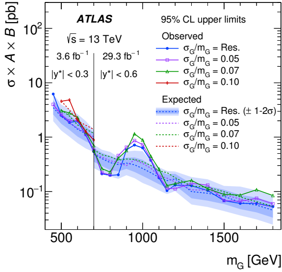
Figure 6: The 95% credibility-level observed upper limits on \sigma \times A \times B for two jets for a hypothetical signal producing a Gaussian contribution to the observed m_{jj} distribution. The limits are shown for a relative width \sigma_G/m_G corresponding to a width equal to the detector mass resolution. While the vertical axis is shared by the two selections, the signal acceptance varies, thus the two sets of limit points relate to two different interpretations of \sigma \times A \times B (see text for some typical acceptance values used for models considered by this search). The different y^* selections are described in the text.
