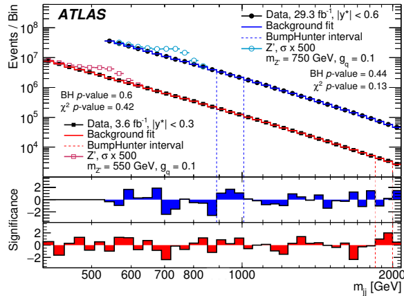
Figure 4: The reconstructed dijet mass distribution (filled points) for events in the |y^*| < 0.3 and |y^*| < 0.6 signal regions. The solid lines depict the background estimate obtained by a sliding-window fit. Overall agreement between the background estimate and the data is quantified by the \chi^2 p -value. The most discrepant localized excess in either signal region identified by the BumpHunter algorithm is indicated by the vertical lines. The open points show two possible signal models. The lower panels show the bin-by-bin significances of differences between the data and the background estimate, considering only statistical uncertainties.
