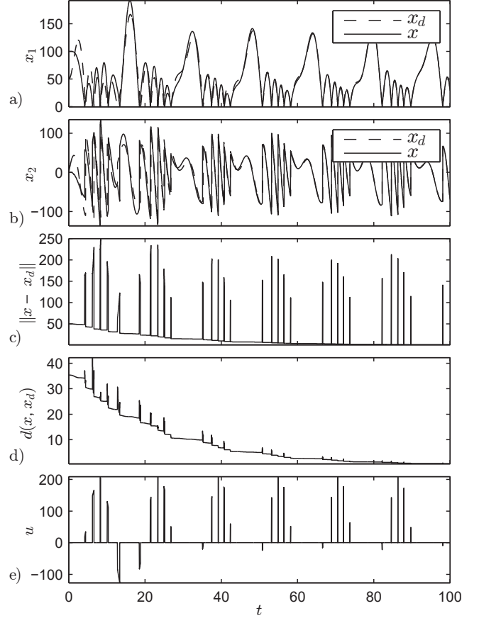
Figure 3. a) and b) Reference trajectory x_d and plant trajectory x for the dissipative mechanical system and periodic forcing. c) Euclidean tracking error. d) Distance function (2). e) Control force u .
