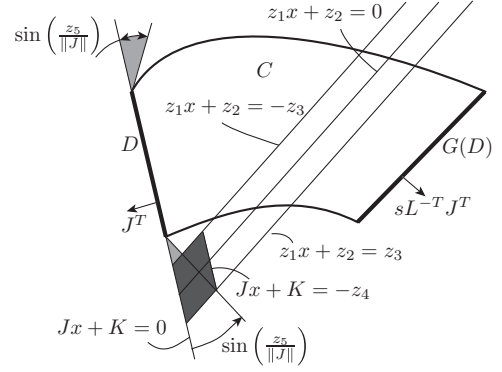
Figure 1. Pictorial illustration of the phase space of (11) when Assumption 3 is satisfied. The second and third bullet of this assumption imply that the intersection between C and the domains depicted in dark gray and light gray, respectively, is empty.
