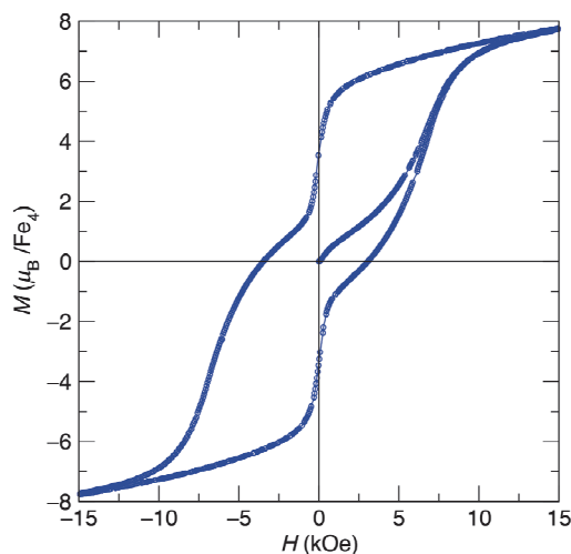
Figure 3. Hysteresis loop at 1.8 K for [\text{Fe}_4(\text{N}=\text{CPh}_2)_6] ( 1 ) showing magnetization vs. applied field cycling from \pm 70 kOe at a sweep rate is 50 \text{ Oe}\cdot\text{s}^{-1} .
