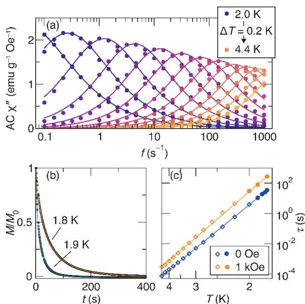
Figure 4. (a) Imaginary part of the AC susceptibility of 1 at zero field as a function of excitation frequency and temperature. The lines shown are fits to the generalized Debye model. (b) DC saturation-decay measurements used to characterize the relaxation at low temperatures, where the relaxation times are long. (c) Arrhenius plot of the relaxation times in zero field (blue) and 1 kOe field (orange). The fits shown are to Eq. 1.
