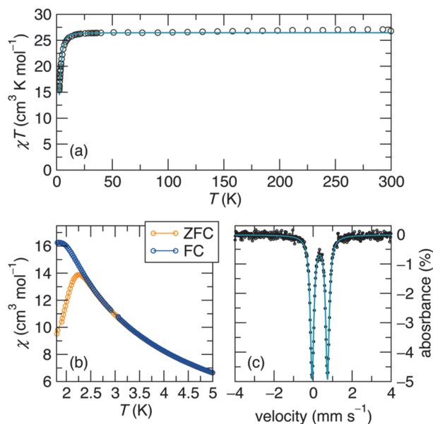
Figure 2. (a) Susceptibility multiplied by temperature of 1 measured at a field of 5 kOe, demonstrating that the S = 7 ground state persists to room temperature. The teal line is the fit to the spin Hamiltonian \hat{H} = D\hat{S}_z^2 + g_{\text{iso}}\mu_B S \cdot H , where S = 7 , D = -0.32 \text{ cm}^{-1} , and g = 1.94 . (b) Zero-field cooled and field-cooled low-temperature susceptibility taken at 500 Oe, showing a bifurcation at 2.4 K for the measurement sweep rate of 1 \text{ K} \cdot \text{min}^{-1} . (c) Zero-field ^{57}\text{Fe} Mössbauer spectrum collected at 90 K (black dots) and fit (teal line).
