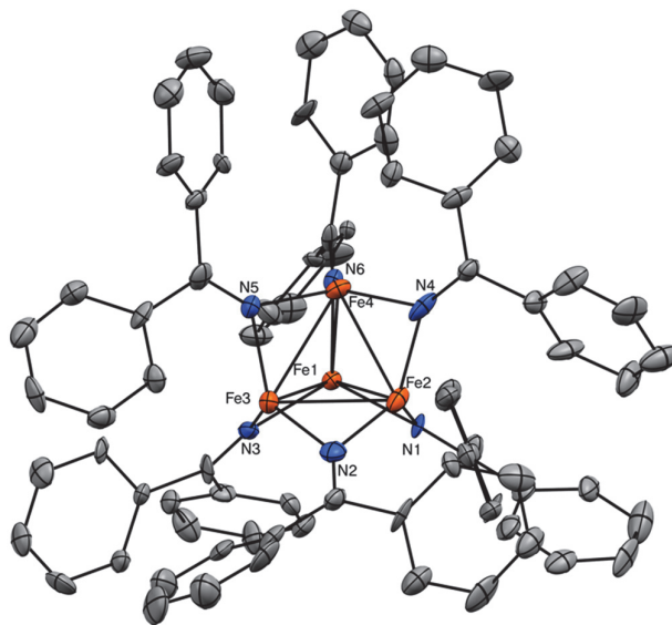
Figure 1. ORTEP diagram of one independent molecule of 1 with 50% probability ellipsoids. Hydrogen atoms, toluene solvates, and a second molecule of 1 are omitted for clarity. Color legend: Fe = orange; N = blue; C = grey.
