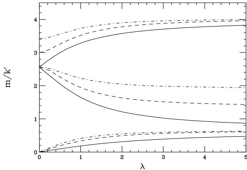
Figure 9: The spectra for the top KK tower. The horizontal axis is \lambda = y_u H , and the vertical axis is the masses in units of k' . The solid, dashed and dot-dashed lines are for (c_L, c_R) = (0.4, 0.4) , (0.4, 0.1) and (0.4, -0.2) , respectively.
