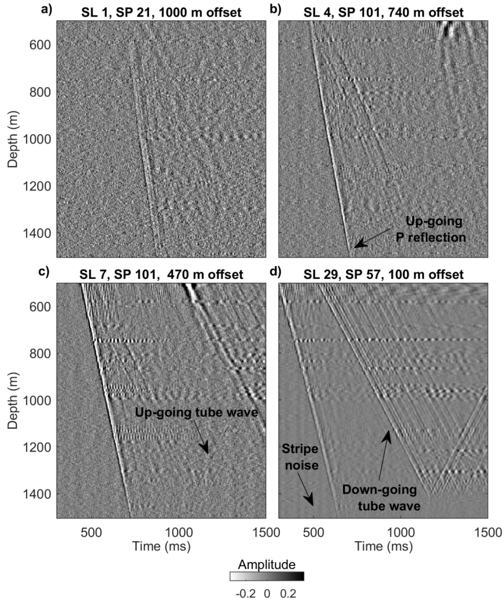
Example of shots acquired with DAS VSP on tubing, no signal processing applied after correlation. Displayed shots range from offset of 1000 m (a), 740 m (b), 470 m (c), and 100 m (d).
