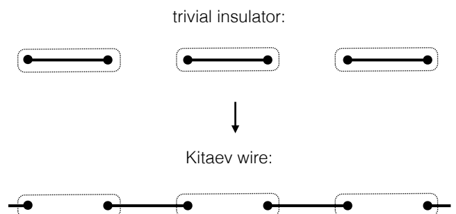
FIG. 1: Majorana SWAP model.
