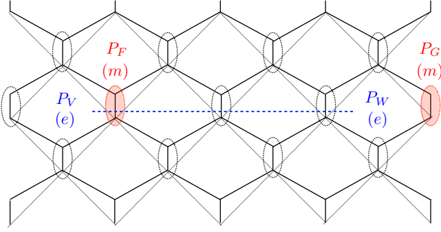
FIG. 12: The action of U_F(T) turns an e string operator into an m string operator.
