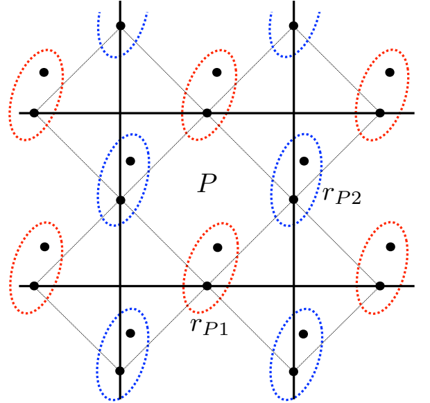
FIG. 11: Toric code with additional ancilla spins
