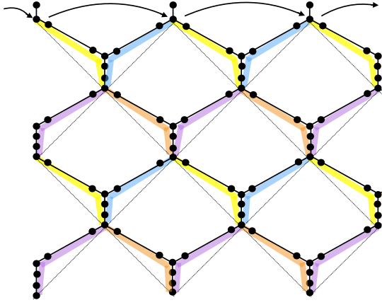
FIG. 9: Action of Floquet unitary on the edge
