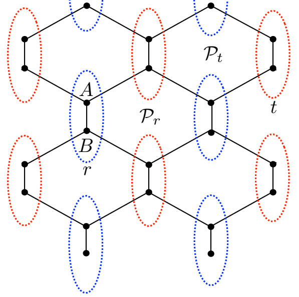
FIG. 7: Honeycomb model. During the Floquet evolution, the observable \mathcal{P}_t associated with red supersites picks up an Aharonov-Bohm phase \mathcal{F}_{P_t} associated with the \mathbb{Z}_2 -flux through plaquette P_t located to the left of t . Similarly, for blue supersites, the relevant plaquette is located to the right of r .
