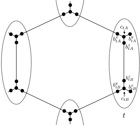
FIG. 8: Majorana representation of honeycomb model
