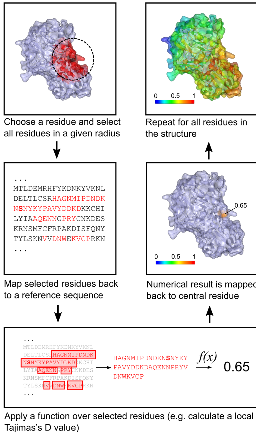
Figure 1. Overview of the structural mapping with spatial averaging approach as used in the Python BioStructMap package. For any given residue within a PDB structure, all residues within a specified radius of the given residues are identified. The location of these residues within a given reference sequence is then found, with the assumption that user-provided data will be aligned to this reference sequence. Using selected residues and the corresponding subset of user-provided data, a function is called, returning (usually) a numerical value. For example, this function may return the mean of the respective data. Note that the provided data and the mapping function may take a diverse number of forms. This includes functions which apply some statistical test over a multiple-sequence alignment of genetic sequences (e.g. Tajima's D). In this case, the function would apply the statistical test over the subset of codons which code for the selected residues. The returned value is then assigned to the original residue in the PDB structure. This process is repeated for all residues within the PDB structure. Results can be viewed as a heatmap displayed over the PDB structure.
